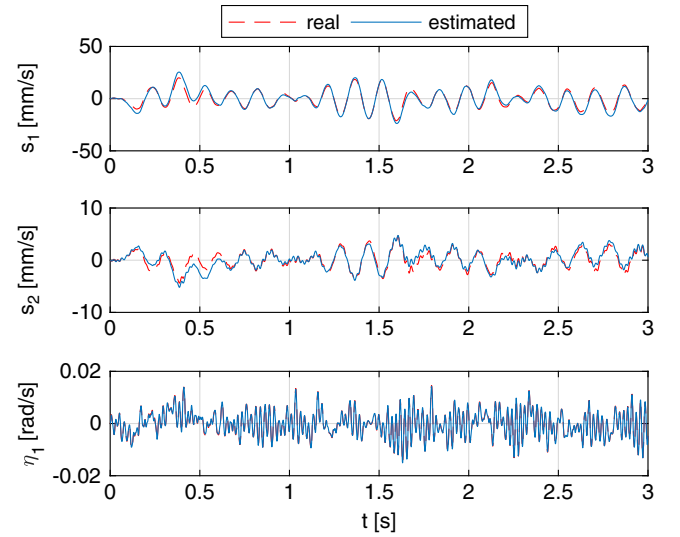
Fig. 9 Real and estimated deformation velocities.
