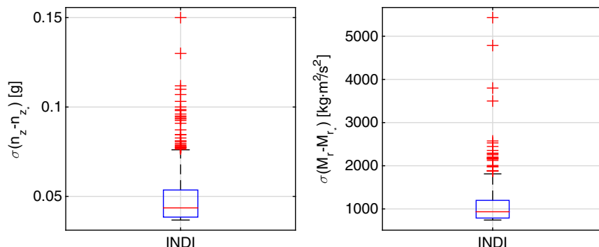
Fig. 30 Box plot of a Monte Carlo simulation of the closed-loop system subjects to model uncertainties.
