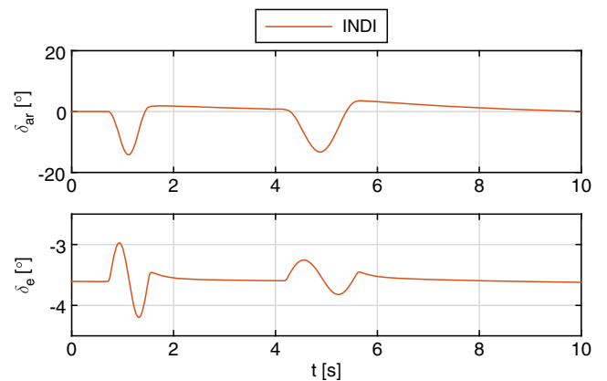
Fig. 22 Control inputs in a gust field.
