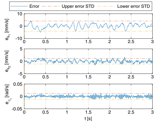
Fig. 10 Deformation velocity estimation errors (STD, standard deviation).
