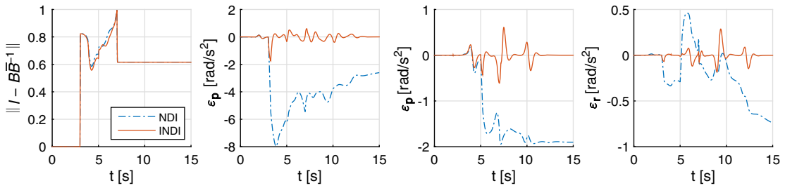
Fig. 8 Value of \|I - \mathcal{B}\mathcal{B}^{-1}\| and the residual errors in the fourth actuator fault scenario.
