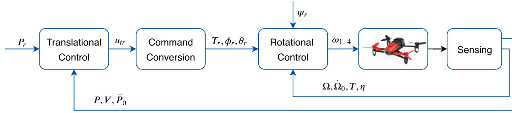
Fig. 2. Block diagram for control structure.
