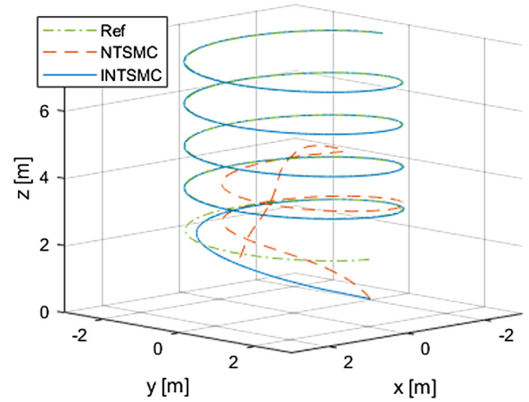
Fig. 13. 3D trajectory responses in the presence of uncertainties, disturbances, and successive actuator faults at t = 10, 15, 20, 25 s (Scenario 3).
