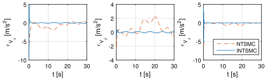
Fig. 12. Responses of \epsilon_{V_x} , \epsilon_{V_y} , \epsilon_{V_z} using NTSMC and INTSMC in Scenario 2.
