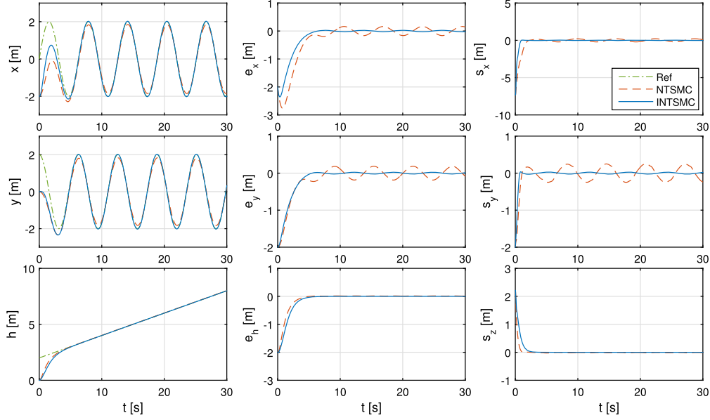
Fig. 4. Position responses in the presence of model uncertainties (Scenario 1).
