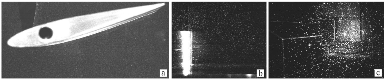
Fig. 3 Raw images from the three experiments. a NACA 0012 airfoil; b near-wake of a truncated cylinder; c near-wake of the Ahmed body
