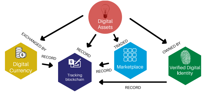
Figure 1: The four pillars of UniCon, our infrastructure to manage digital assets. The tracking blockchain maintains a tamper-proof history of digital assets.
