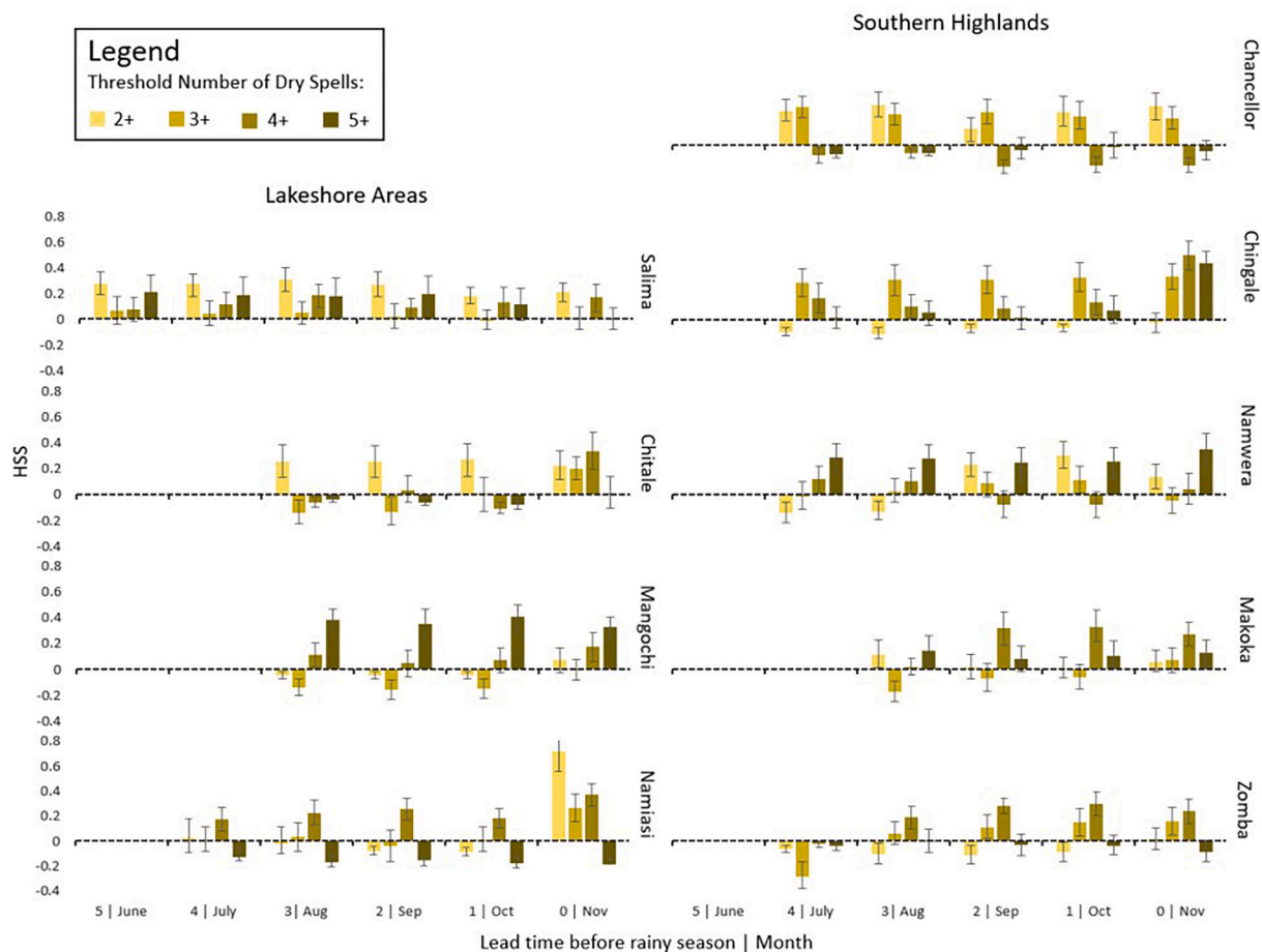
Fig. 5. Heidke Skill Score (HSS) of k-fold cross validation results for stations in Lakeshore Areas (left) and Southern Highlands (right), at different thresholds for number of dry spells (2+, 3+, 4+ and 5+). The error bars indicate the 5 th and 95 th percentiles of the HSS. Skilful forecasts are observed when the HSS is above zero, including the error bar.
