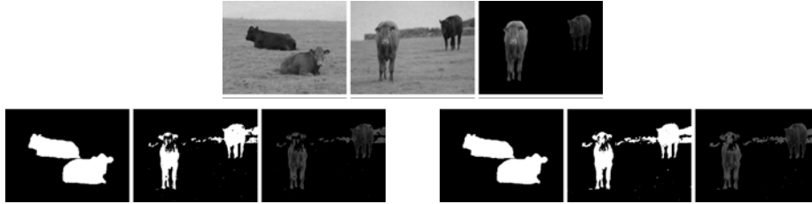
(a) \hat{\mu} = 150, \sigma = 10^3 , error = 5.54 %, time = 6.6 sec.
