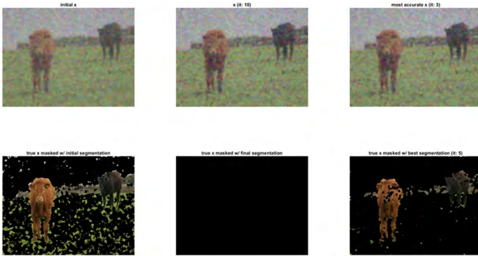
Figure 6.6: Results after 10 iterations of (6.9) using the linearised (6.9a), and using parameter set-up (II).
