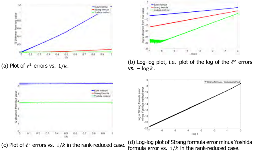
Figure 5.5: Comparison of the \ell^2 error from approximating e^{-\tau A}u via the semi-implicit Euler method (blue), Strang formula (red), and Yoshida method (green) approximations for e^{-\tau A}u on the graph built on the image in Fig. 5.4. For (a) and (b), K = |V| . For (c) and (d), K = \sqrt{|V|} . The gradient of the line in (d), excluding outliers for small k , is 2.000. In (c), the green and red lines are both plotted but cannot be distinguished by the eye.
