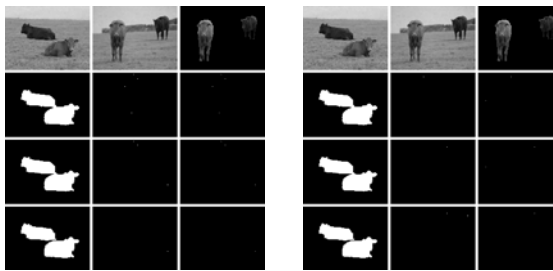
(g) \hat{\mu} = 150, \sigma = 10^4 , error: 12.8122%, time: 6.5 sec.
