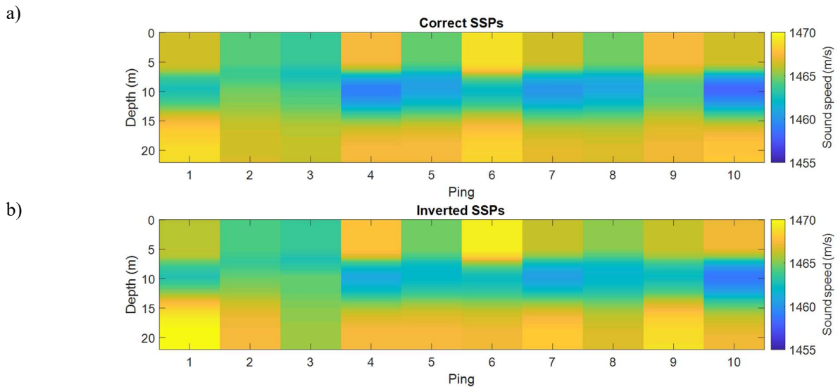
Figure 4. The correct SSPs (a) and the inverted SSPs (b) for all pings along track 1 ( x = 30 in Fig. 1a).
