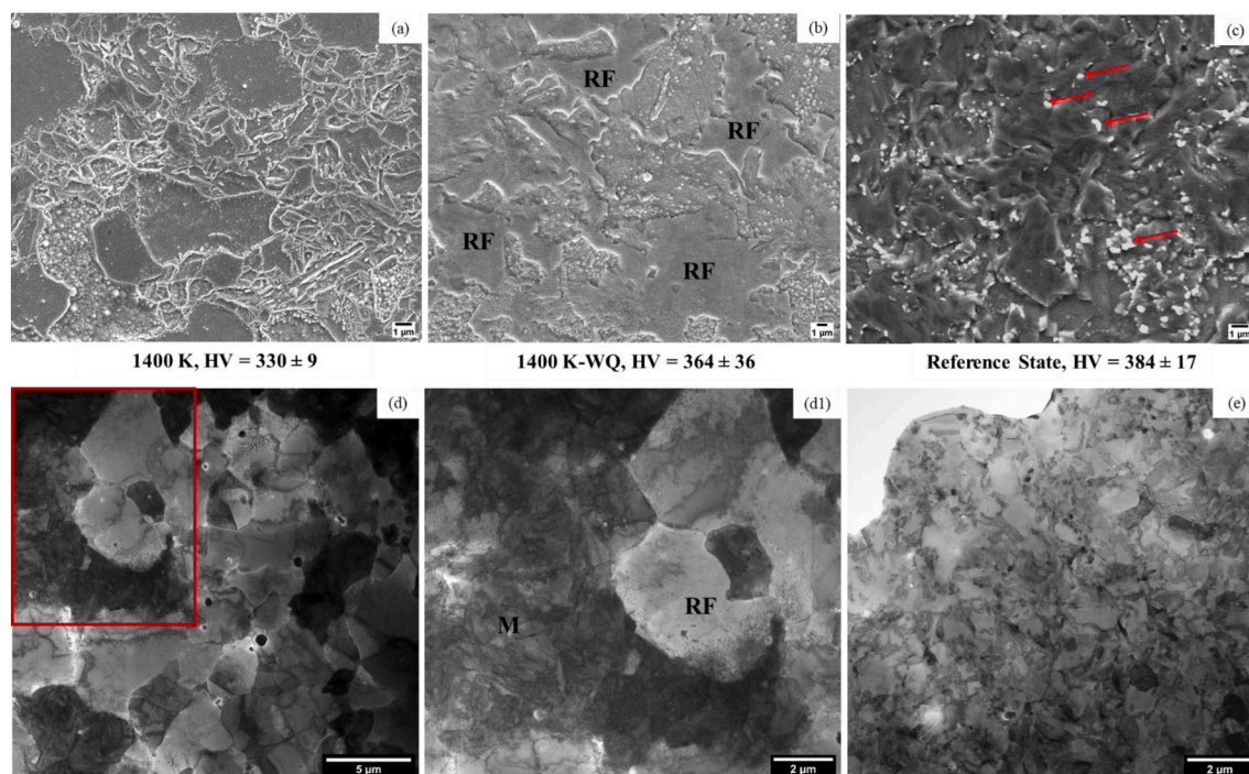
Fig. 2. Secondary electron micrographs of the 0.3% \text{Y}_2\text{O}_3 ODS Eurofer steel and respective average Vickers hardness in the (a) condition of annealing at 1400 K, followed by furnace cooling (1400 K-FC), (b) annealed at 1400 K and water quenched (1400 K-WQ) and (c) reference state, with red arrows indicating \text{M}_{23}\text{C}_6 carbides. (d) and (d1) Bright-field micrographs showing the martensite (M) and recrystallized ferrite (RF) in the sample 1400 K-FC and (e) reference state. (For interpretation of the references to colour in this figure legend, the reader is referred to the web version of this article.)
