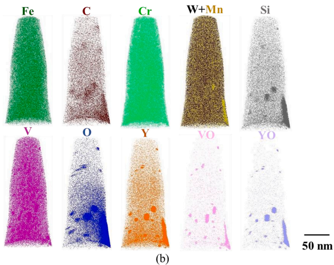
Fig. 4. Compositional maps of representative reconstructions of 0.3% \text{Y}_2\text{O}_3 ODS Eurofer samples (a) in the reference state and (b) annealed at 1400 K-FC.
