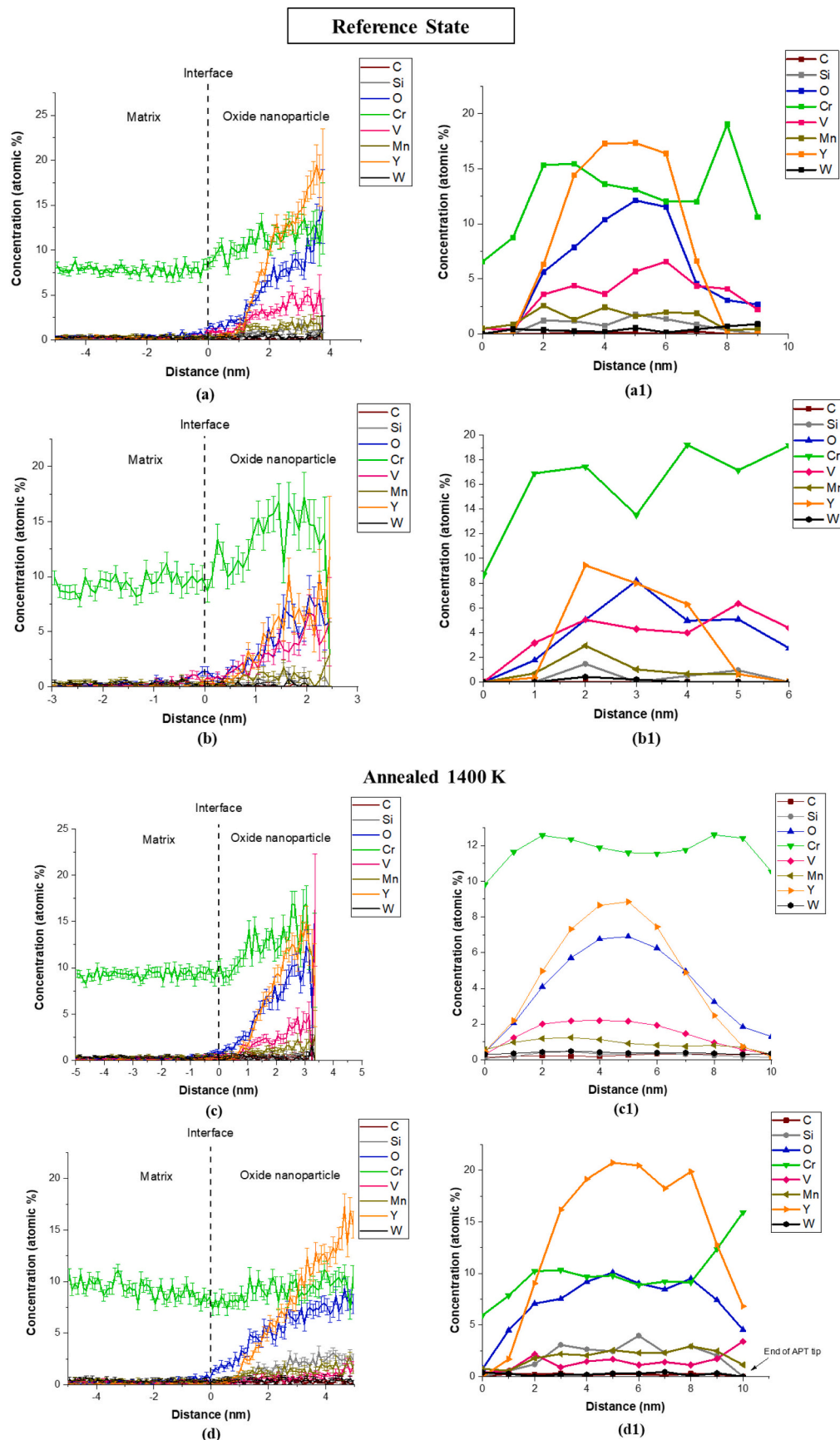
Fig. 7. (a),(a1) and (b),(b1) Proxigram along 1% Y isosurface and respective concentration profile along ROI of two representative oxide nanoparticles present in the reference state sample. (c),(c1) and (d),(d1) Proxigrams and concentration profiles along ROIs of two particles present in the sample annealed at 1400 K-FC.
