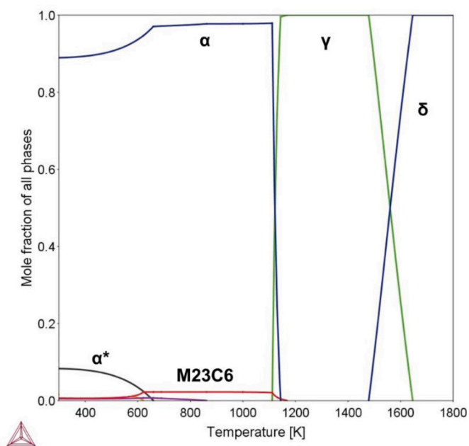
Fig. 1. Mole fraction of phases that can be present in the 0.3% \text{Y}_2\text{O}_3 ODS Eurofer steel, calculated for its composition without the oxide particles. Composition used: Fe-0.1C-9.18Cr-1.97 W-0.196 V; Thermo-Calc version and database: 2018a and TCFe9 Steels/Fe-alloys v9.0.
