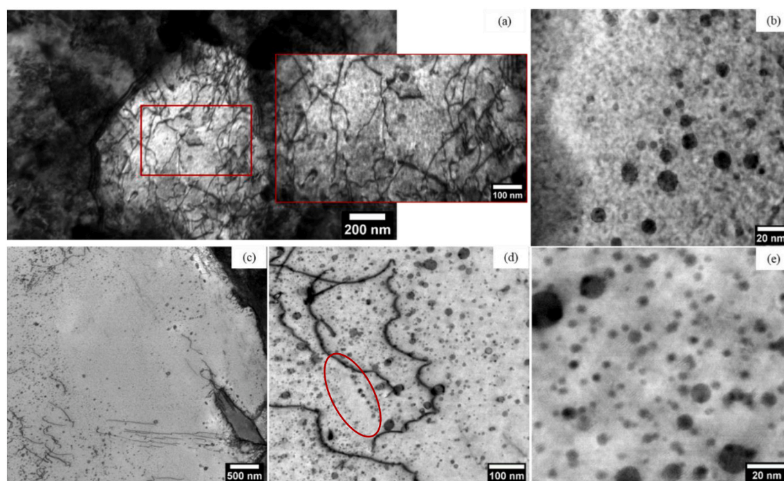
Fig. 3. Bright-field micrographs of the 0.3% \text{Y}_2\text{O}_3 ODS Eurofer showing Y-O based nanoparticles and their distribution in the matrix. In (a) and (b) the material is in the reference state and in (c), (d) and (e) in the condition 1400 K-FC. In (d), a band free of oxide nanoparticles is encircled in red. (For interpretation of the references to colour in this figure legend, the reader is referred to the web version of this article.)
