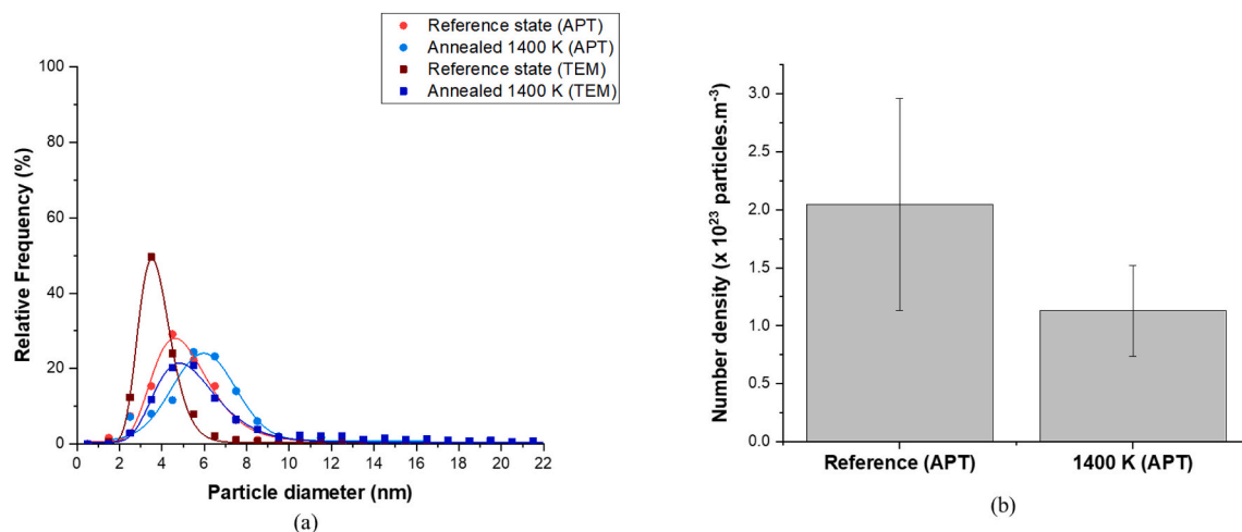
Fig. 5. (a) Particle size distributions and (b) number density of oxide nanoparticles calculated for the 0.3% \text{Y}_2\text{O}_3 ODS Eurofer steel in the reference state and annealed at 1400 K-FC, using TEM and APT.
