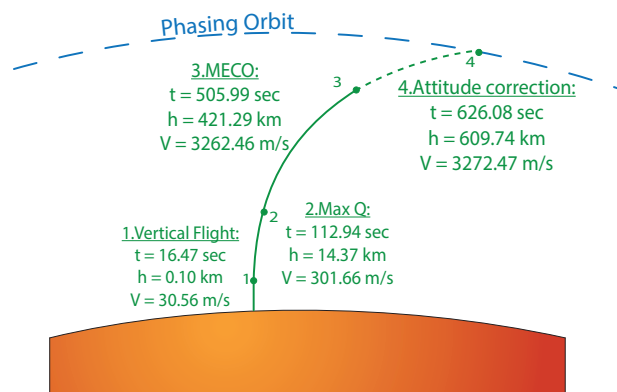
Figure 2. Ascent Profile.
