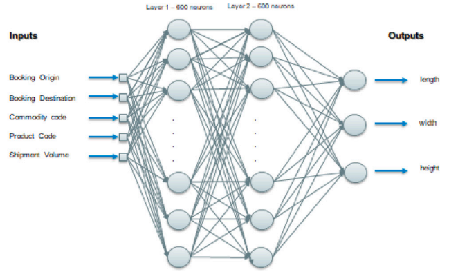
Fig. 5. MLP architecture.
