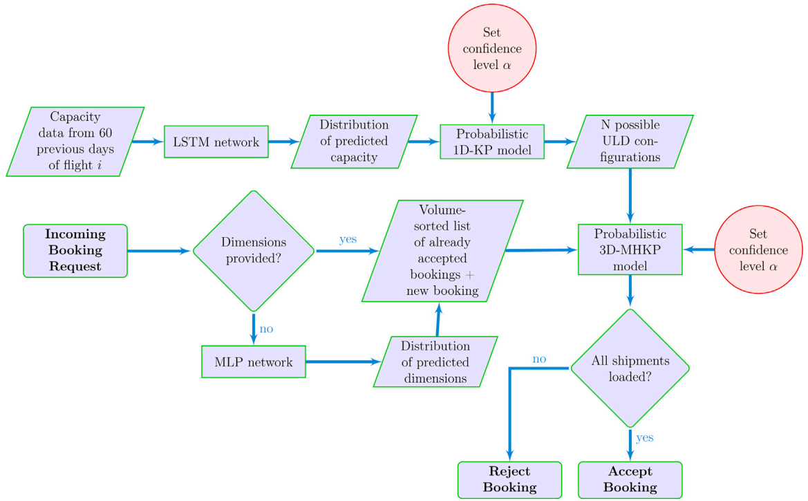
Fig. 13. Flowchart of the decision-making process defining the booking acceptance/rejection strategy.
