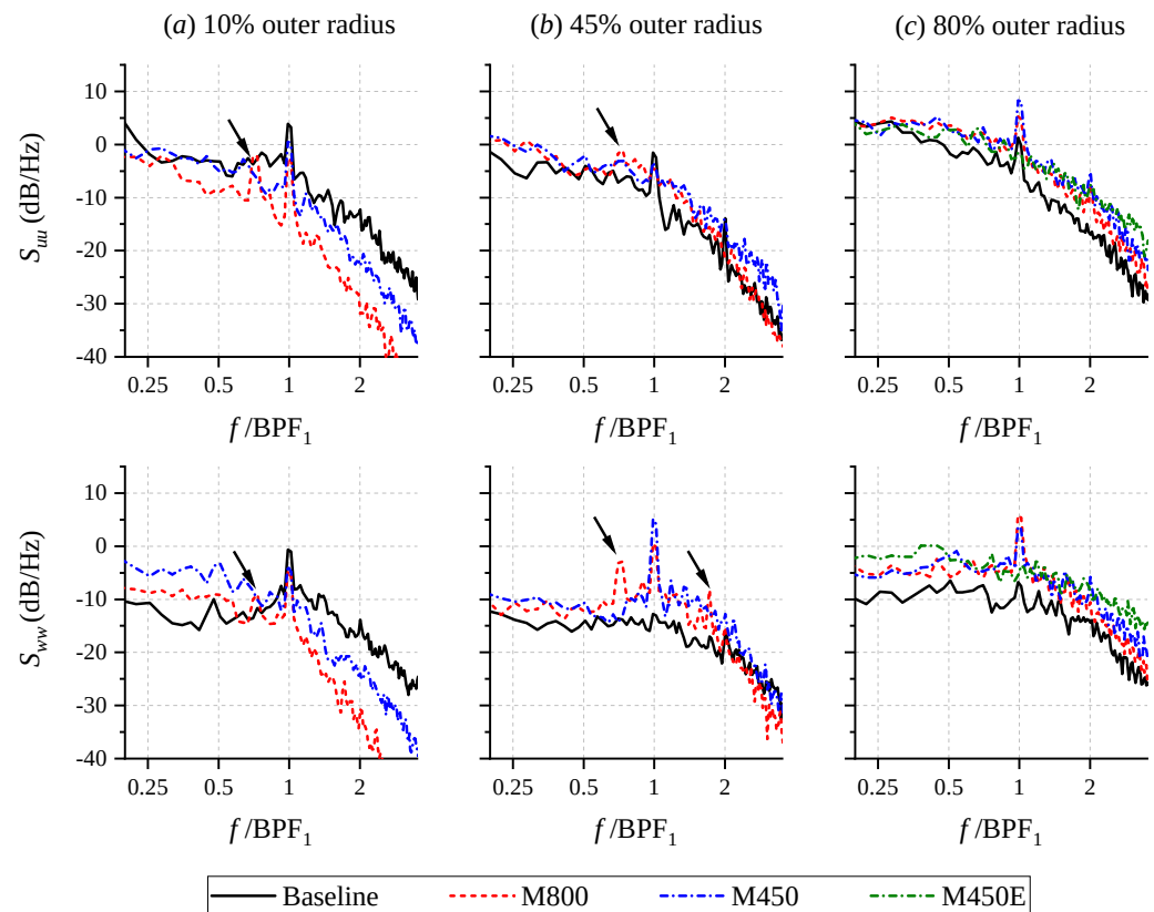
Figure 13. Plots of axial ( S_{uu} ) and tangential ( S_{wv} ) velocity fluctuations spectra at a height of 50 mm (0.23c) above the OGV TE. The power spectral density is normalized against a reference velocity of 1 m/s. The arrows in (a,b) indicate narrowband velocity fluctuations components that are unrelated to the BPFs.
