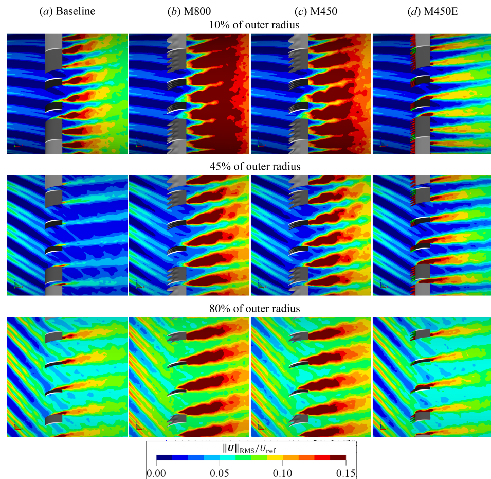
Figure 12. (Side view) Contours of phase-locked standard deviation of velocity magnitude ( ||\mathbf{U}_{\text{RMS}}|| ) at the different radial sections ( top —10 %, middle —45 %, and bottom —80 % of the outer radius) in the fan stage.
