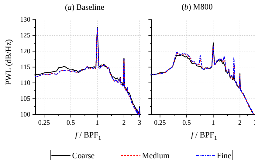
Figure 6. The variation of the sound power level (PWL) of the SDT fan stage against the grid resolution level.
