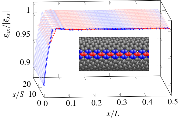
(c) (20,0) zigzag
