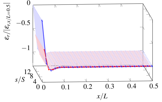
(b) (12,12) armchair
