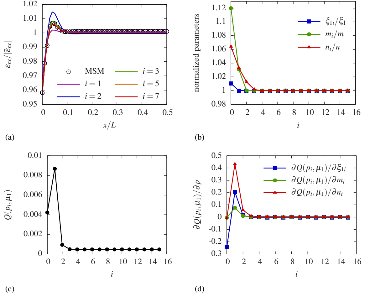
Figure 9: Convergence pattern of the initial k -th step (i.e. \mu_k = \mu_1 ) for the (12,12) armchair SWCNT: (a) normalized nonlocal axial strain field approximating the MSM results (only few iteration steps are displayed), (b) normalized values of the nonlocal parameters \xi_1 , m and n , (c) the cost function and (d) its derivatives with respect to p ( i refers to the iteration number).
