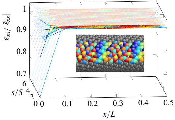
(e) (18,6) chiral
