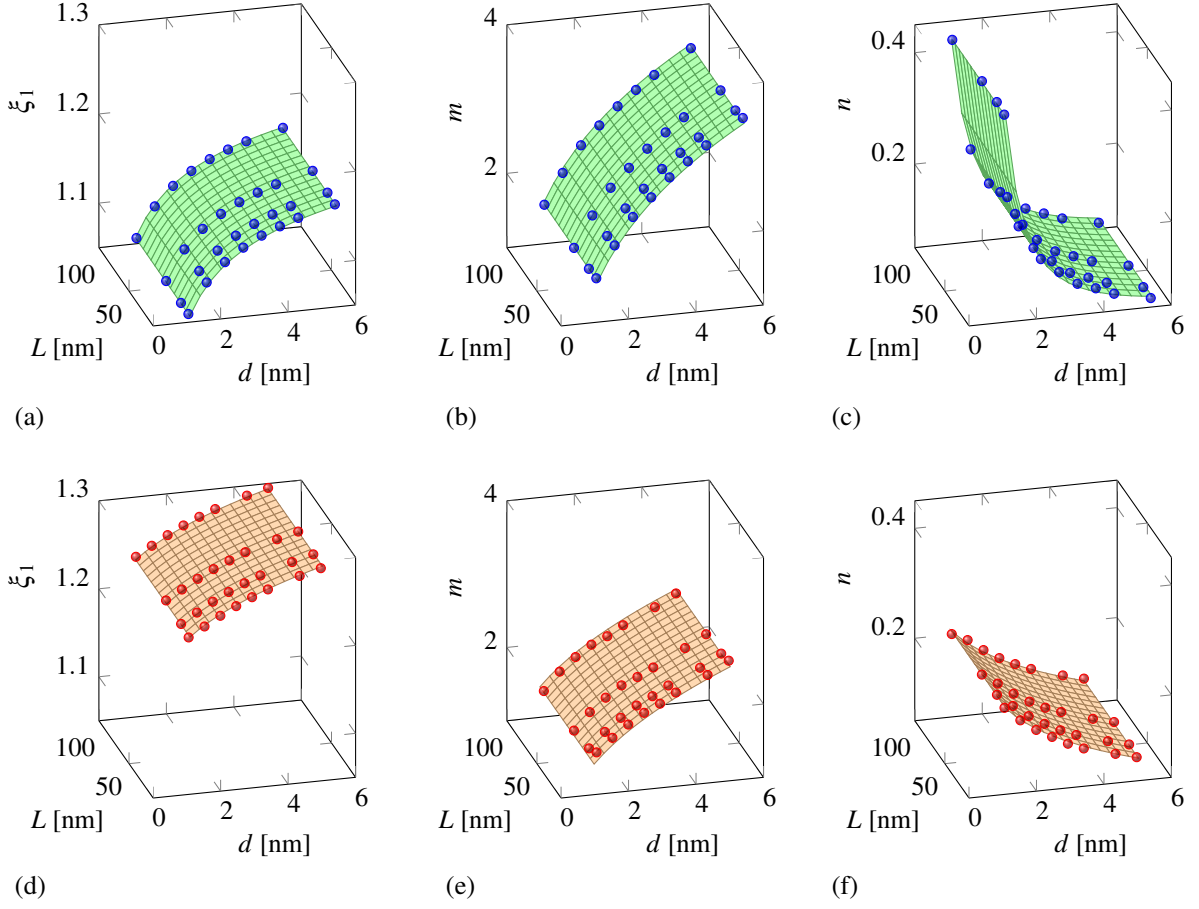
Figure 10: Nonlocal parameters \xi_1 , m and n for (a)-(c) (n_1, n_1) armchair and (d)-(f) (n_1, 0) zigzag SWCNTs calculated with the parameter estimation procedure (filled markers) and corresponding approximating surface.
