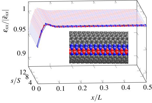
(a) (12,12) armchair
