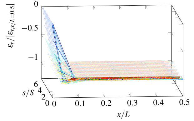
(f) (18,6) chiral
