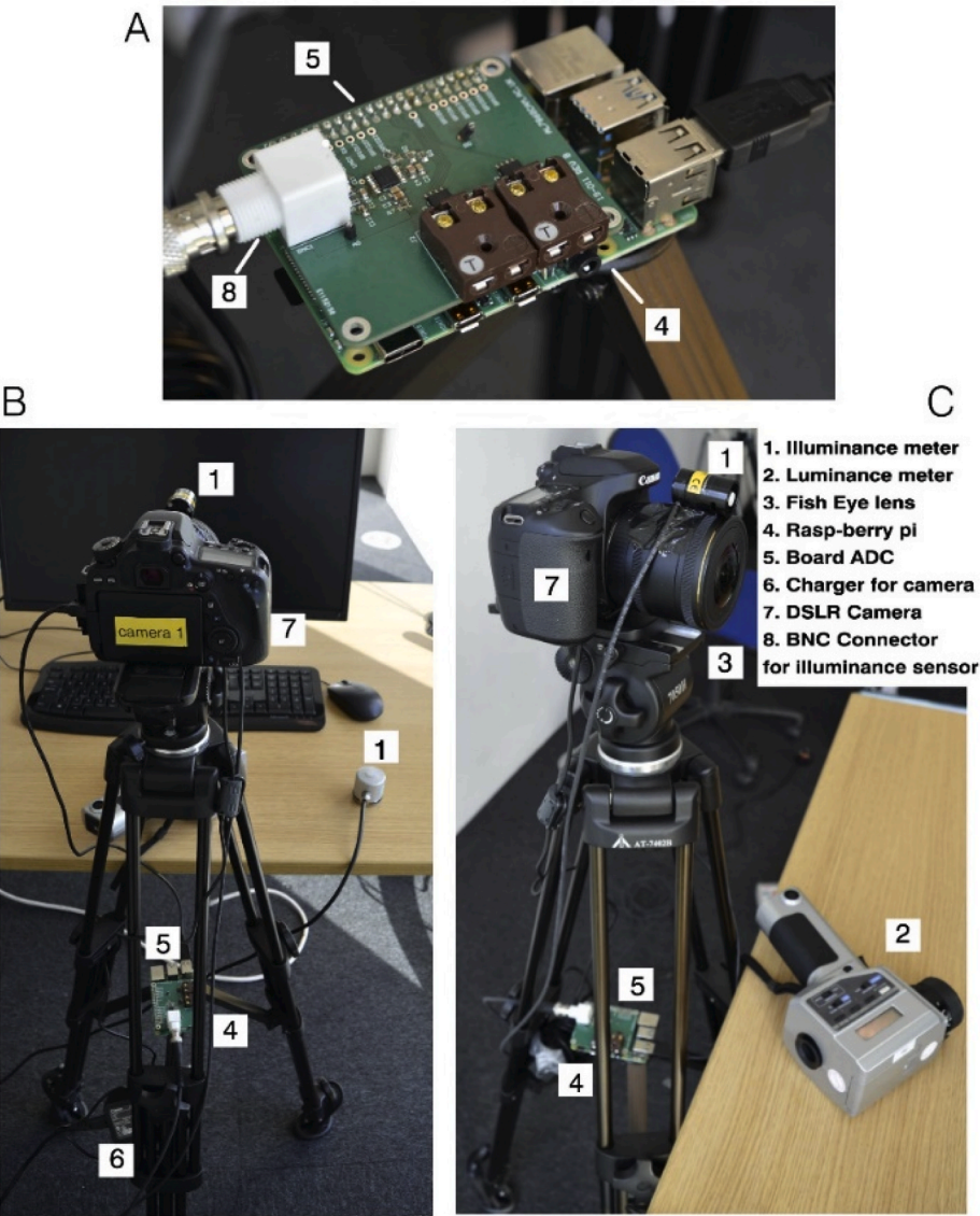
Fig. A1. Glare monitoring setup, located behind the occupant (after Luna-Navarro and Overend [18]).
