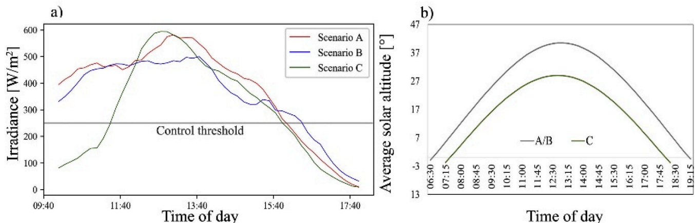
Fig. C1. Outdoor conditions during the façade test scenarios: a) external incident vertical irradiance; b) average solar altitude (retrieved from Ref. [51]).
