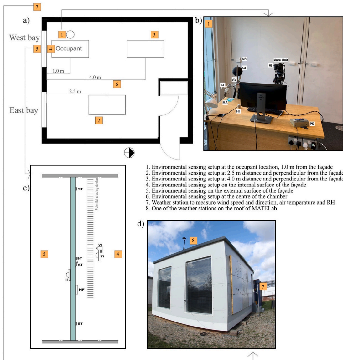
Fig. 3. Environmental sensing setup during the experiments (after [19]) (for label descriptions, see Table 3): a) plan view with location of the environmental sensing setups across the floor plan; b) view of the environmental sensing setup at the occupant desk location (1); c) section view of the environmental sensing setup on the internal (4) and external side (5) of the façade; d) view of two of the weather stations (7,8). The characteristics of the sensors are reported in Appendix A.
