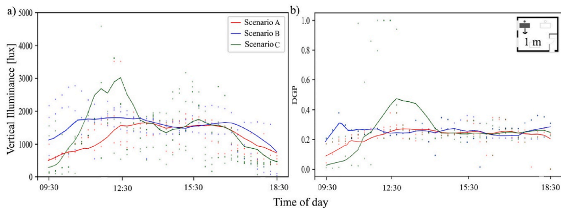
Fig. 12. a) Average vertical illuminance at the eye level and b) daylight glare probability (DGP) at 1.0 m from the façade on a typical day in September for façades A and B, and in October for façade C. The viewpoint was fixed and parallel with respect to the façade, the measurements were taken with a frequency of 15 min.
