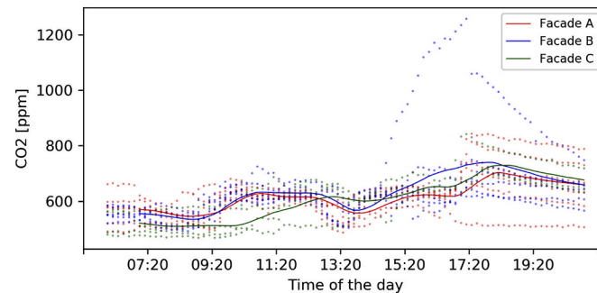
Fig. D2. Monitored levels of CO 2 throughout the day.
