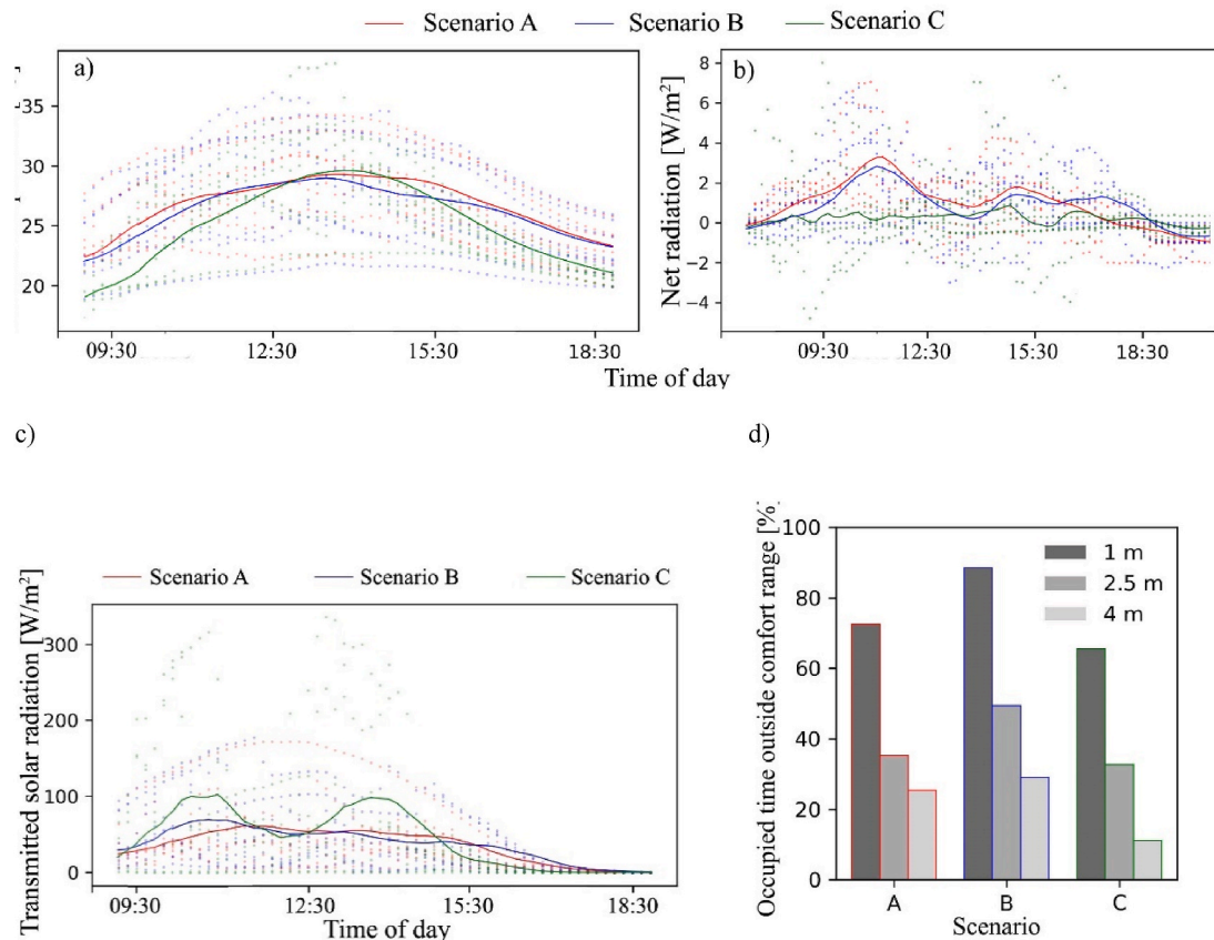
Fig. 10. Radiant heat gains from façade. a) Internal surface temperatures and average surface temperature of the glazing; b) net radiation and average net radiation at the occupant position towards the façade; c) transmitted solar radiation and average transmitted radiation for the three scenarios; d) percentage of occupied time when the operative temperature is above the comfort range (operative temperature > 26 °C).
