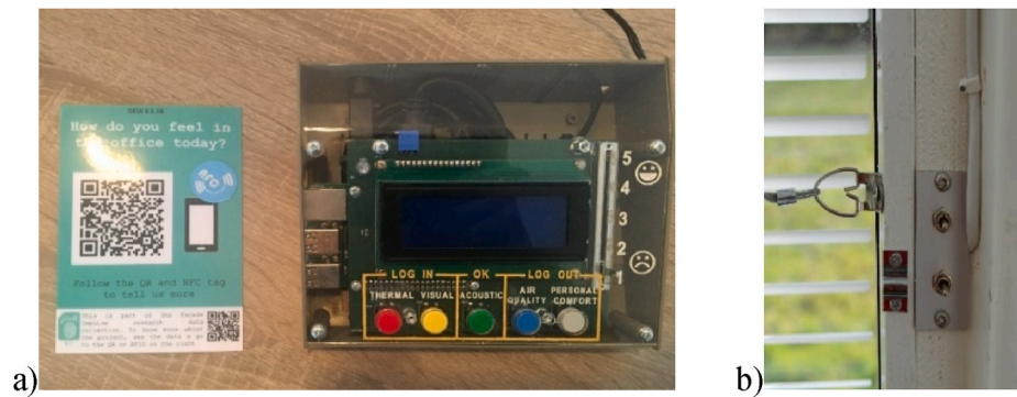
Fig. 5. Occupant interfaces used to solicit feedback. a) On the left, the quick response (QR) code and near-field communication (NFC) tag to open the app on the volunteers' mobile. On the right, the polling station used to gather feedback on discomfort and transient levels of environmental satisfaction, after [19]. b) The switches used by the volunteers to control the blinds.
