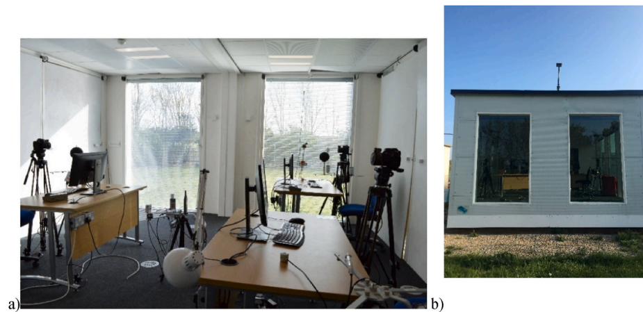
Fig. 1. MATELab. a) Internal view; b) external view of south façade.
