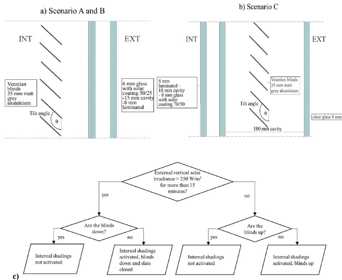
Fig. 2. Key features of the façades tested shown schematically: a) façade investigated in scenarios A and B: DGU with internal venetian blind; b) façade investigated in scenario C: CCF with venetian blind in the cavity. Full specifications are provided in Table 1. EXT and INT refer to the external and internal environment, respectively; c) control algorithm for the automated strategy.
