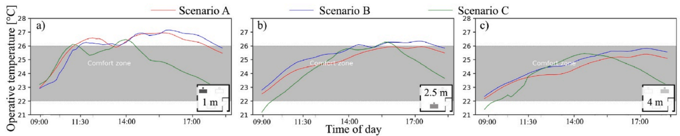
Fig. 9. Average operative temperature for the three scenarios at: a) 1.0 m; b) 2.5 m; c) 4.0 m from façade. The relevant desk location is shown in the inset floor plan.
