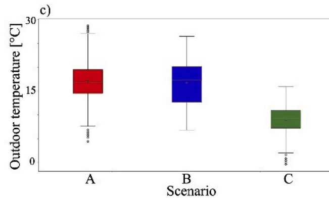
Fig. C2. Plot of the outdoor temperatures during the three scenarios - the coloured rectangles represent the second and third quartiles of the data distribution, the vertical bars indicate the interquartile range, the data points represent the outliers, the cross the average and the horizontal line the median. .
