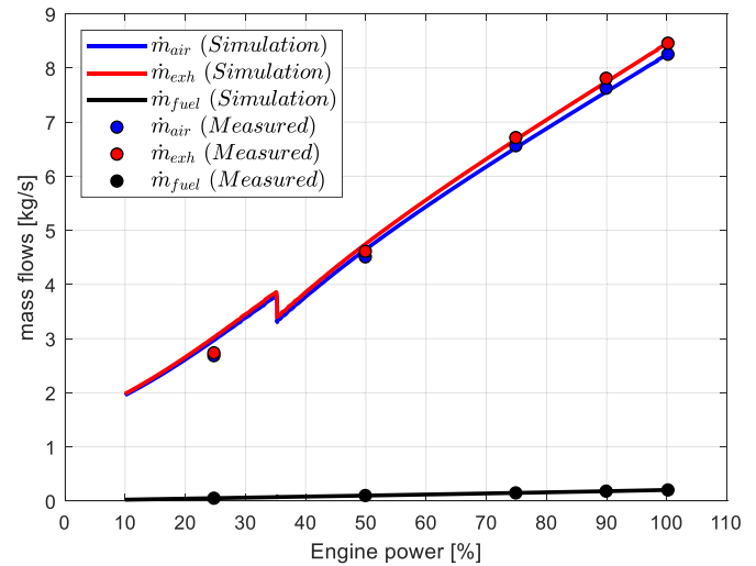
Fig. 10. Mass flows.
