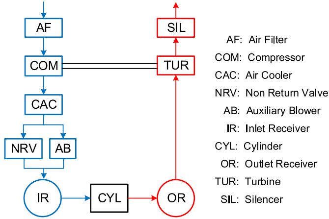
Fig. 4. Layout diagram of MAN6S35ME two-stroke marine diesel engine.
