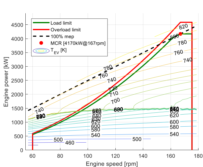
Fig. 24. Exhaust valve temperature T_{EV} (Stationary behaviour).
