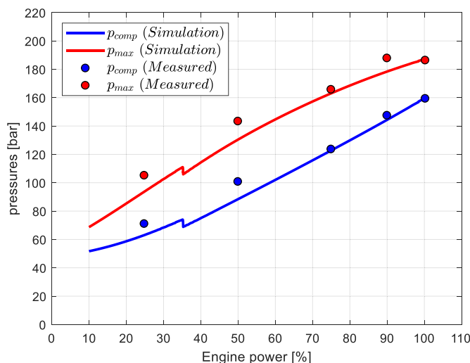
Fig. 14. In-cylinder pressures.
