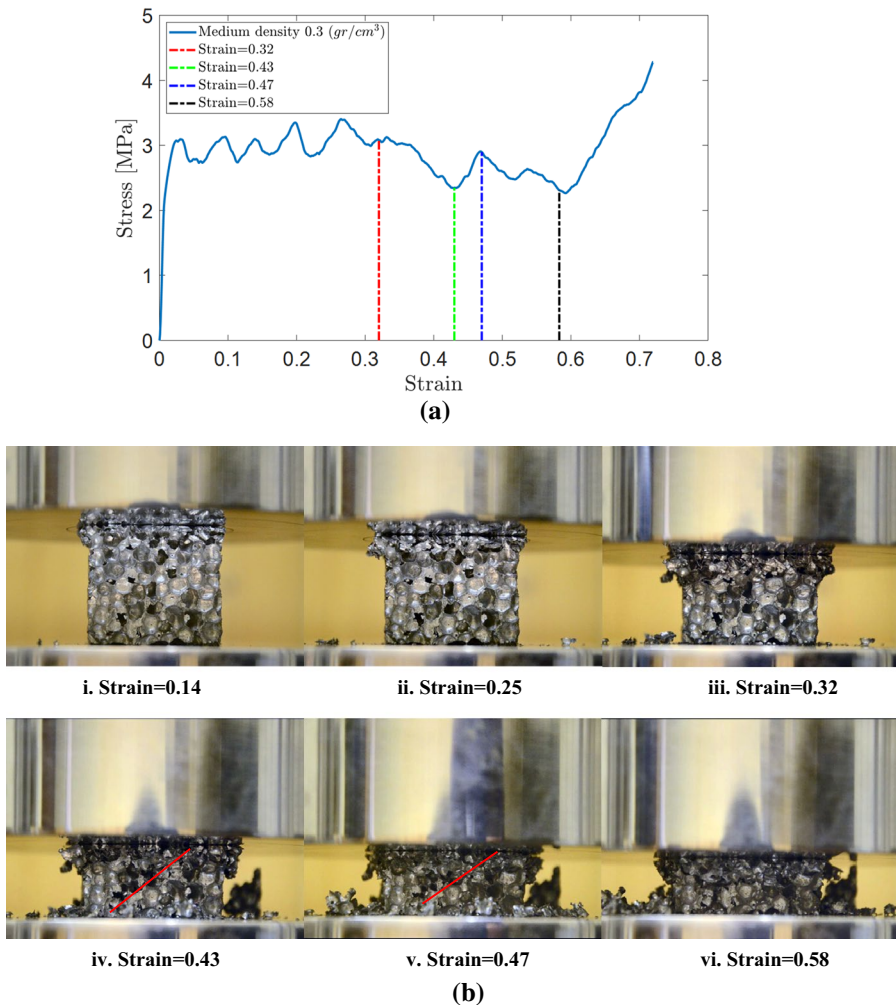
Fig. 6 a Stress–strain diagram and b deformation of the medium-density specimen. The photographs of specimen in (b) is taken at the peaks or troughs of the stress–strain curve of the same specimen shown in (a) , i.e. at strains of 0.14, 0.25, 0.32, 0.43, 0.47, and 0.58. The red lines mark the fracture planes of the specimen
