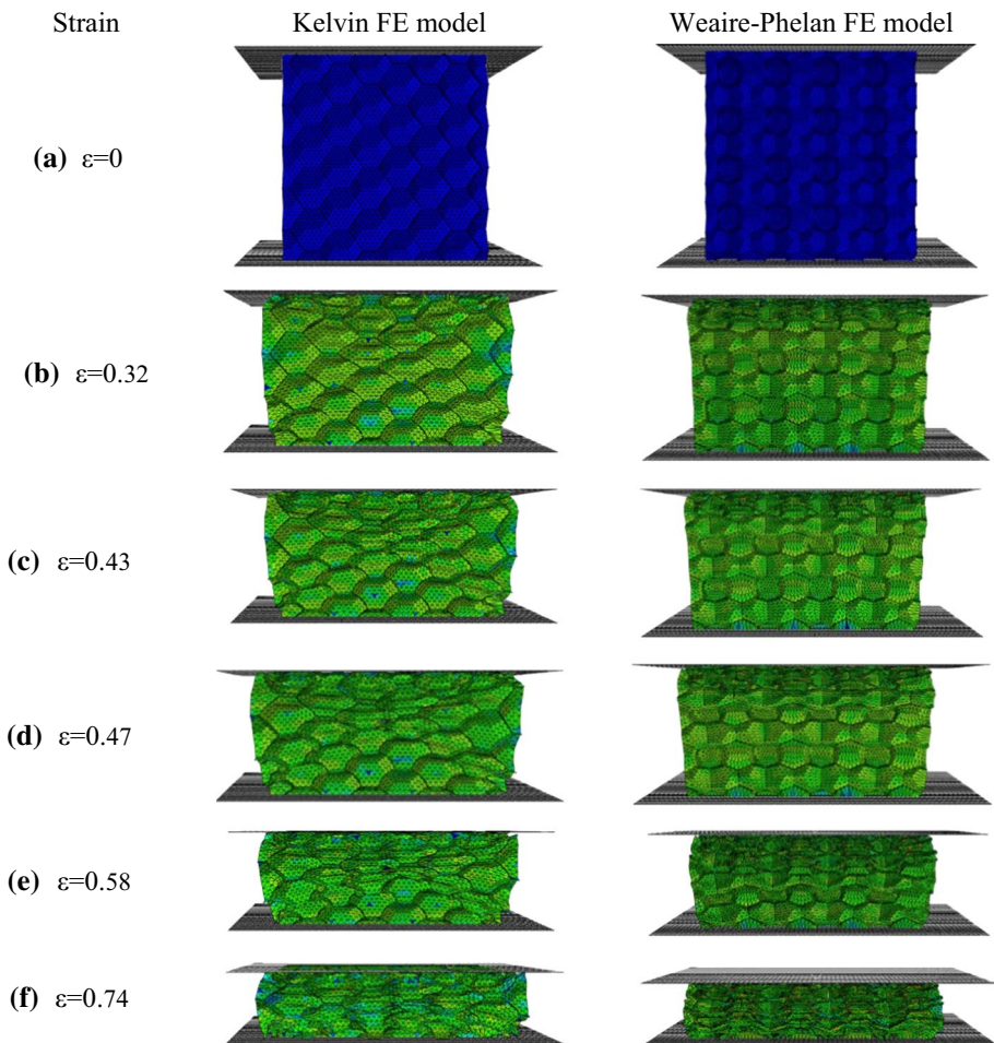
Fig. 10 Stress distribution in the Kelvin and Weaire–Phelan FE models at different strains: a \varepsilon=0 , b \varepsilon=0.32 , c \varepsilon=0.43 , d \varepsilon=0.47 , e \varepsilon=0.58 , and f \varepsilon=0.74
