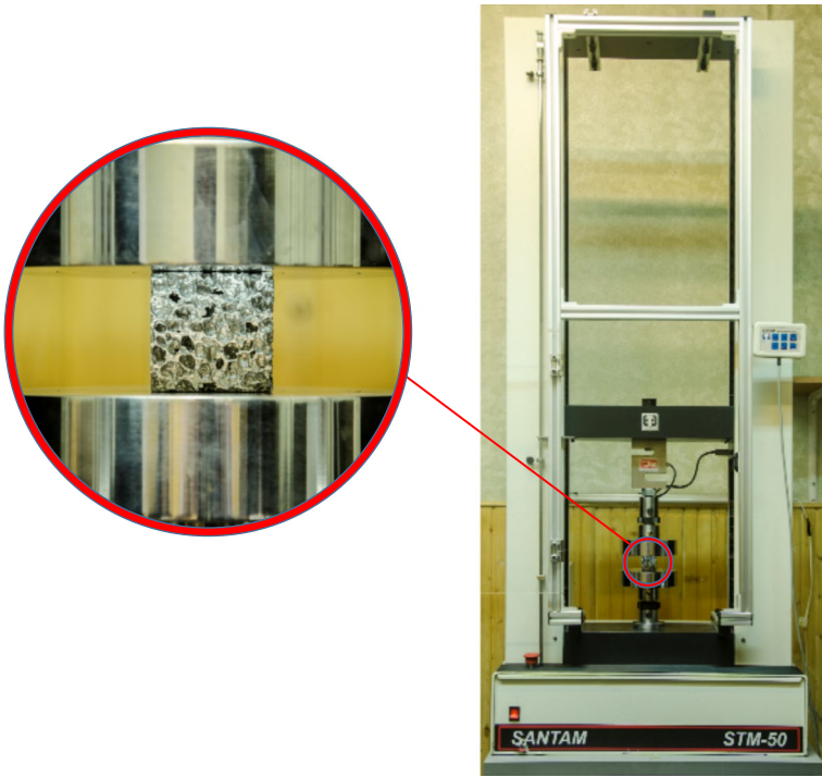
Fig. 2 Compression test device SATNAM STM-50
