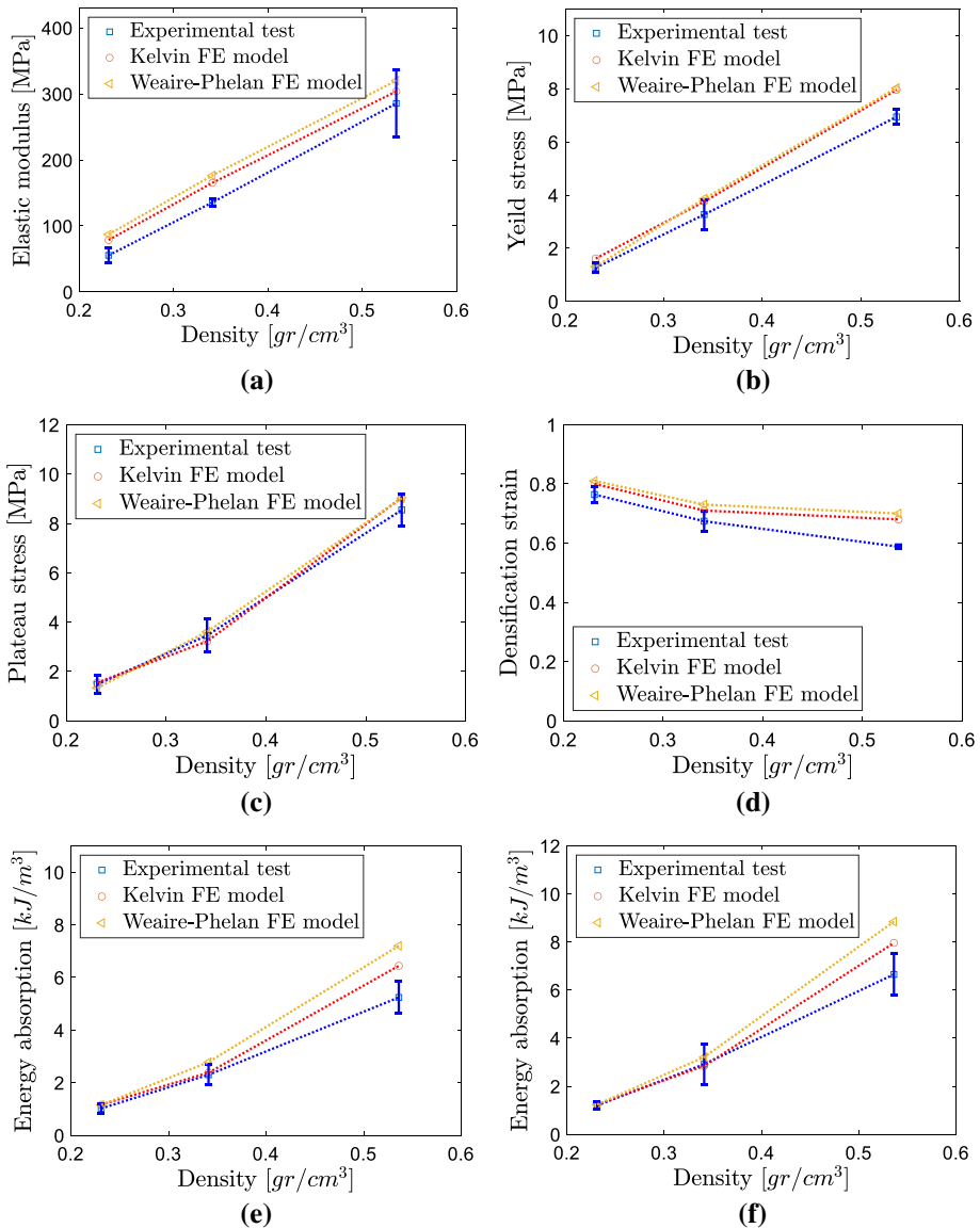
Fig. 8 Variations of mechanical properties of the foam structures with respect to density: a Elastic modulus, b Yield stress, c Plateau stress, d Densification strain, e Energy absorption (strain=0 to densification strain), f Energy absorption (strain=0 to end point of the test)
