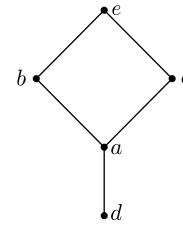
Fig. 1. An example of a circle graph induced by the double-occurrence word adcbaebced .
