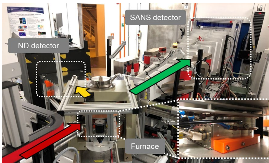
Fig. 3.5. Experimental set-up installed in the Larmor instrument.
