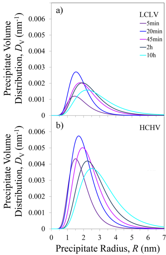
Fig. 2.10. Log-normal volume distribution, D_V , of the VC precipitates in the a) LCLV and b) HCHV steels during annealing at 650 °C for up to 10 h. The curves are based on the R_m , N_p and \sigma values resulted from the fitting of the experimental Q^2(d\Sigma/d\Omega)_{\text{NUC}} results.
