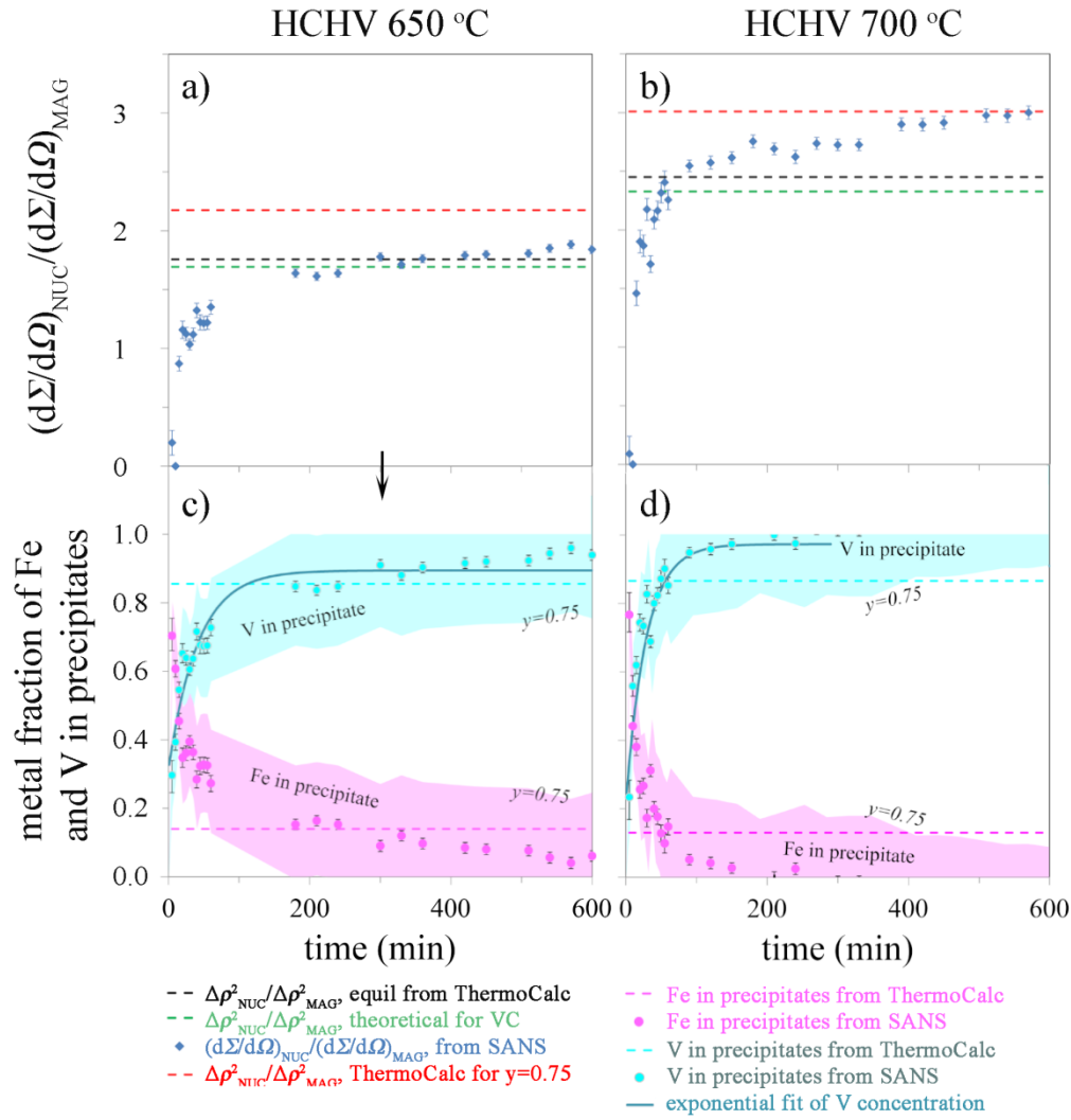
Fig. 4.6. Experimentally observed evolution of the ratio of the nuclear to magnetic scattering cross section of the HCHV steel during annealing a) at 650 °C and at b) 700 °C. The derived precipitate composition evolution is shown in c) and d), respectively. The solid lines in c and d are fits with Eq. (4.9).
