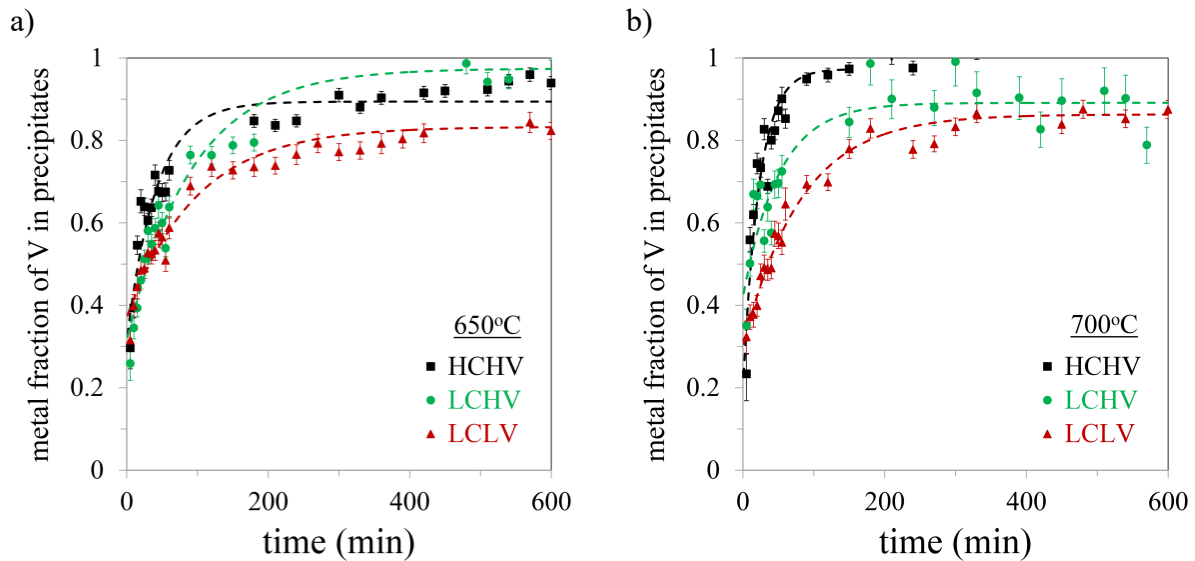
Fig. 4.7. Evolution of the metal fraction of vanadium in the precipitates in the LCLV(▲), LCHV(●) and HCHV(■) steels during annealing at a) 650 °C and b) 700 °C. The marker dots are obtained from the experimental data after solving Eq. (4.8) using the y from ThermoCalc (they are also presented in Figs. 4.4c-d, 4.5c-d and 4.6c-d), and the dashed lines result from the fitting of these data points, i.e., from the fitting of the amount of vanadium in the precipitates.
