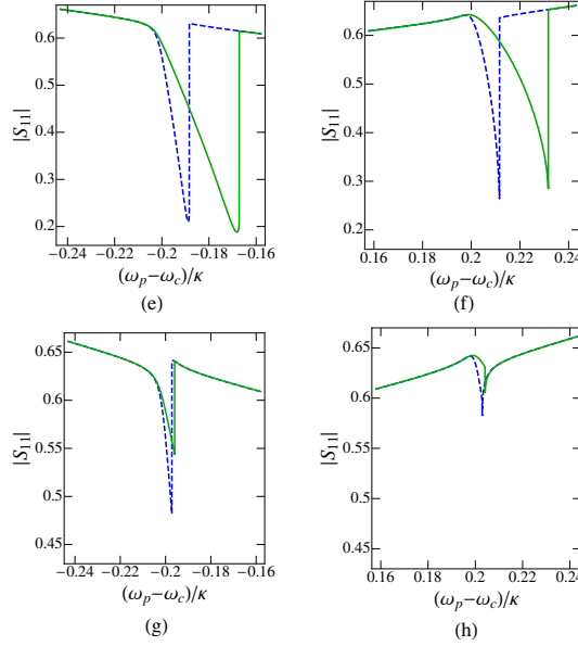
Figure 5.5: OMIA at non-zero detuning. All panels on the left show OMIA for the negative detuning \delta = -0.2\kappa ; all panels on the right are for the same parameters but the positive detuning \delta = 0.2\kappa . (a), (b) The full cavity reflection coefficient in the broad frequency range for the low probe field S_p = 10^4 s^{-1/2} , when the cavity can be considered to be linear. (c), (d) Zoom of the linear OMIA peak. (e), (f) Nonlinear OMIA window of the forward frequency sweep for the two probe fields: S_p = 3 \times 10^6 s^{-1/2} (dashed blue line) and S_p = 5 \times 10^6 s^{-1/2} (solid green line). (g), (h) Nonlinear OMIA of the backward frequency sweep for the same probe fields as in (e) and (f).
