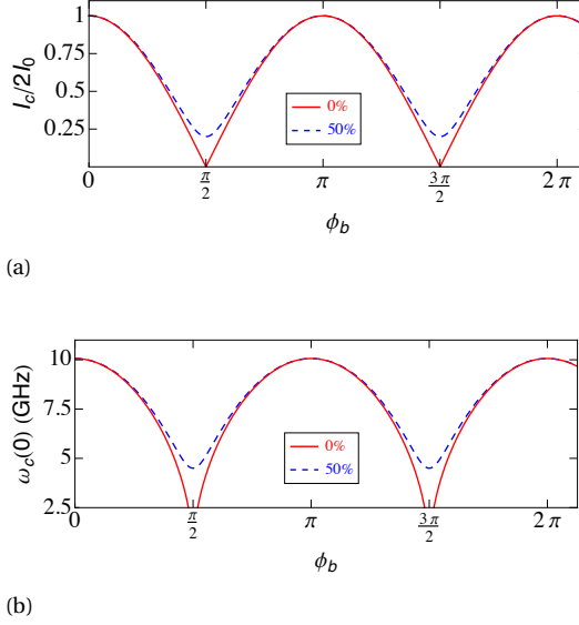
Figure 3.2: (a) The critical current and (b) cavity frequency are plotted as a function of renormalized bias flux of the symmetric and asymmetric SQUID. The cavity frequency of the symmetric SQUID is cut at realistic value of 2.5 GHz.
