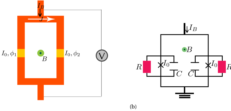
Figure 1.3: (a) Schematic drawing of the dc SQUID. It consists of two Josephson junctions in parallel. The loop is biased by a current I_B and the voltage drop V . (b) Equivalent circuit of the SQUID using RCSJ model.
