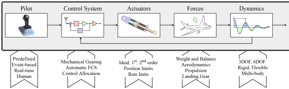
Figure 3.8 Block scheme overview of the PHALANX flight mechanics model.
