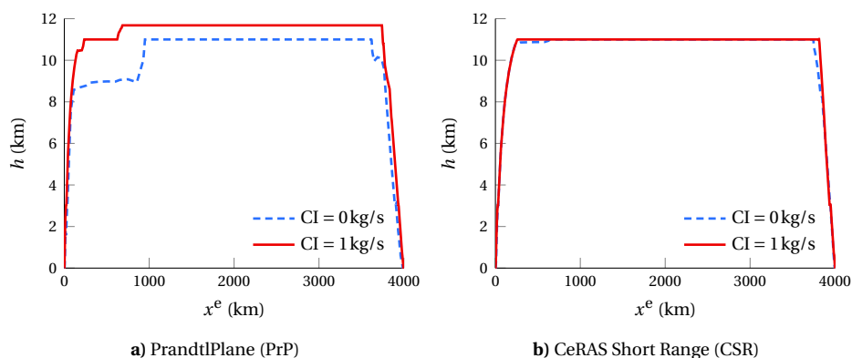
Figure 4.5 Design mission profile for the PrP and CSR, for different CIs.
