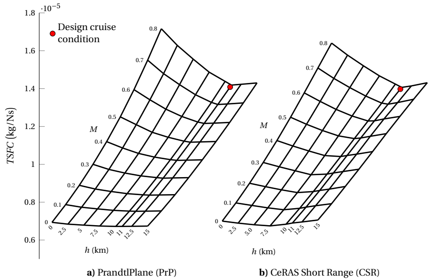
Figure 4.3 Thrust specific fuel consumption carpet plots at max thrust for the PrP and CSR.
