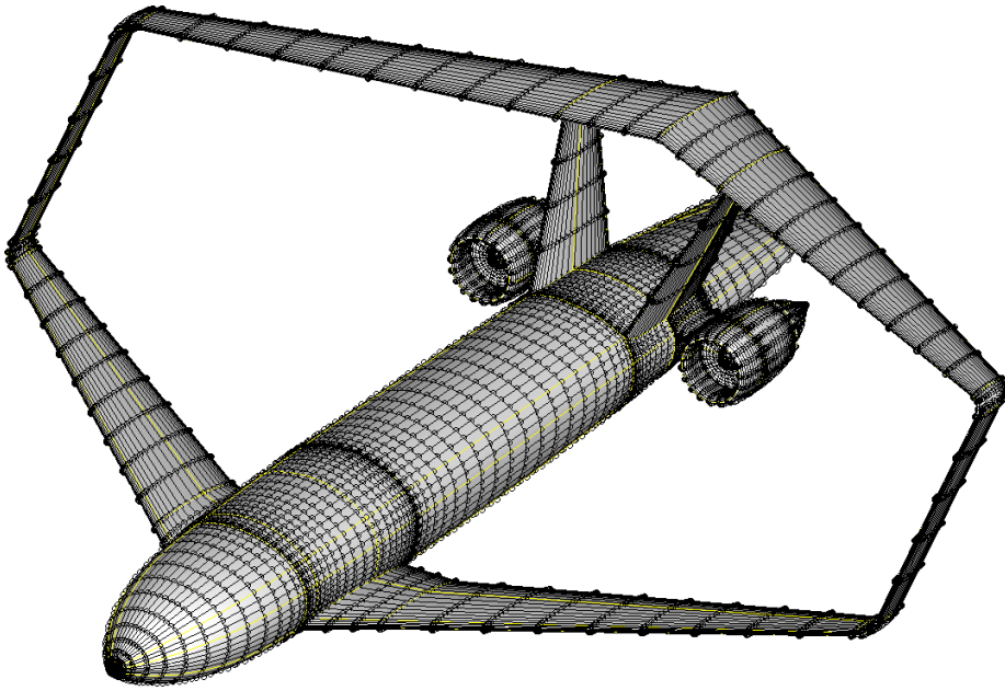
Figure 3.3 Example of a structured surface mesh of the PrP geometry, automatically generated by the MMG.
