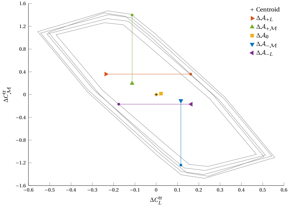
Figure 6.4 Position in Action Space of trim points maximizing control authorities about the pitch and lift axes, for V^{\text{tr}} = 180 m/s.
