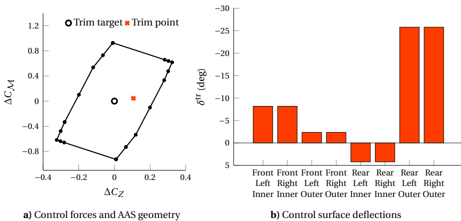
Figure 7.4 Reference trim condition: V^{\text{tr}} = 170 \text{ m/s} , \alpha^{\text{tr}} = -0.46 \text{ deg} .
