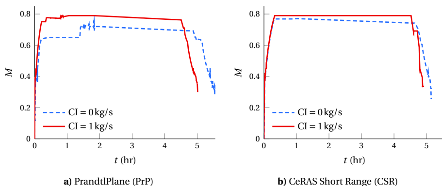
Figure 4.7 Design mission Mach number for the PrP and CSR, for different CIs.
