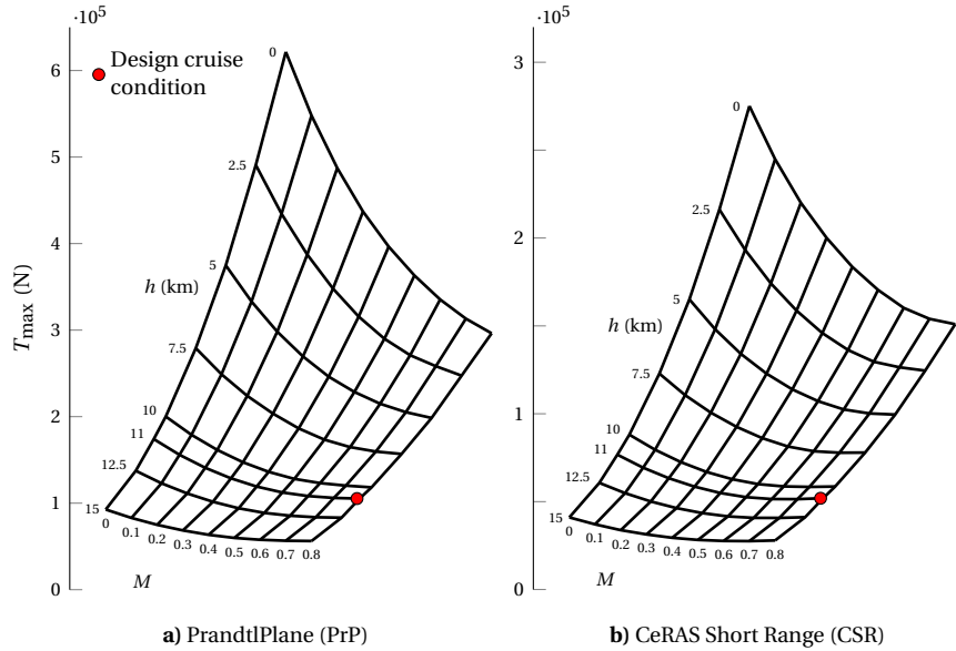
Figure 4.2 Maximum available thrust carpet plots for the PrP and CSR.
