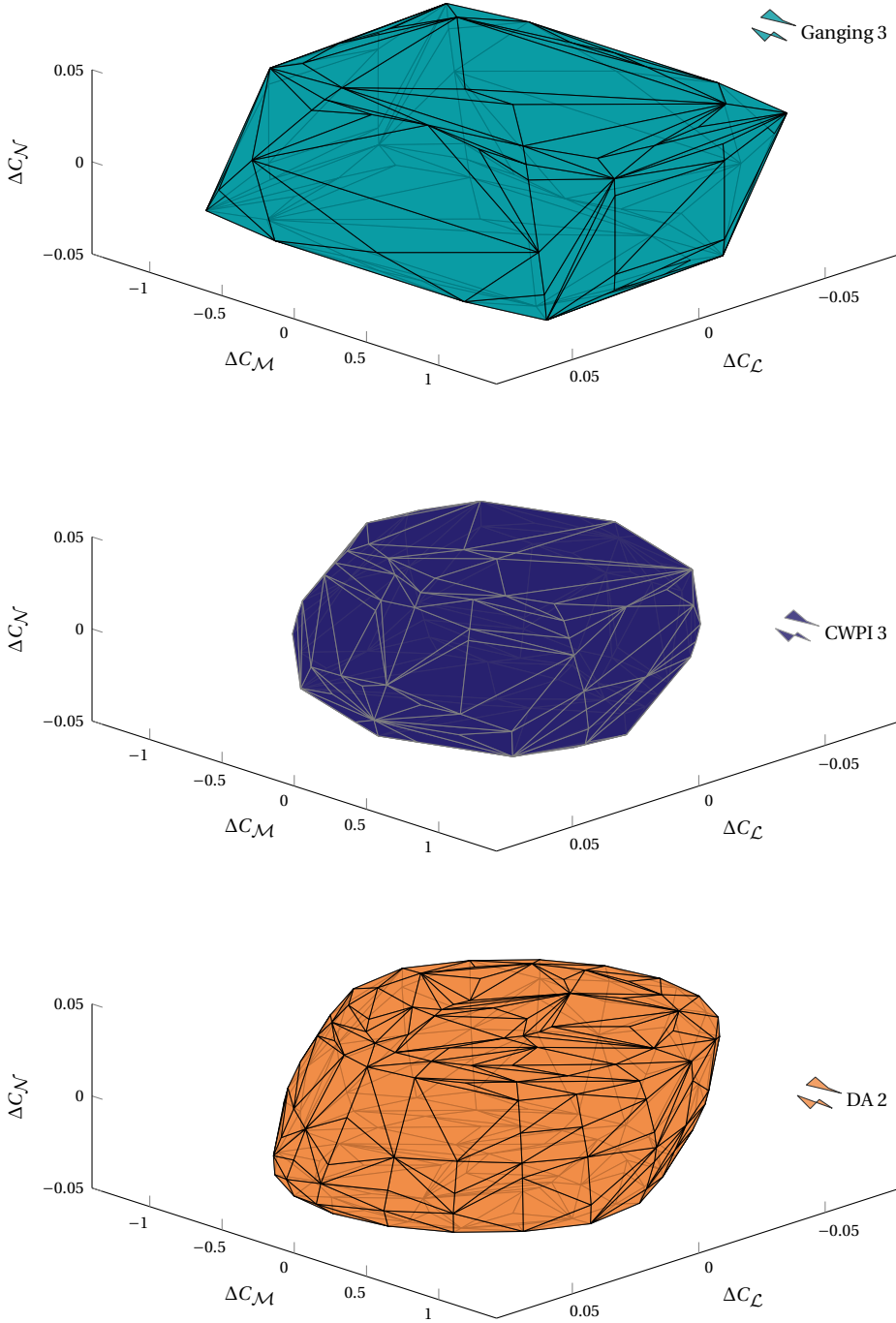
Figure 5.9 Visualization of the AASSs corresponding to the optimal CS layouts obtained with each CA method. The legend entry refers to the CS layouts reported in Table 5.4.
