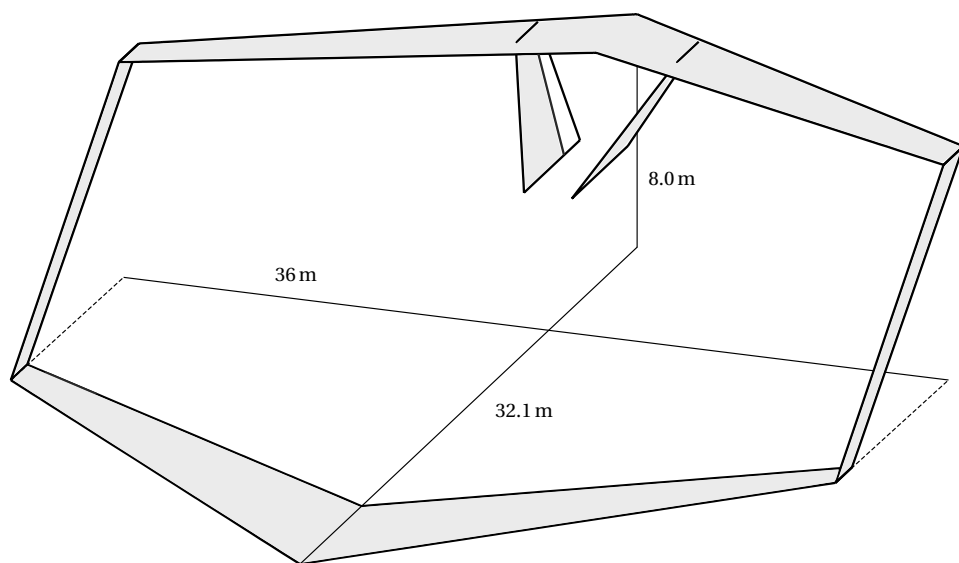
Figure 5.4 Box-wing geometry under investigation.
