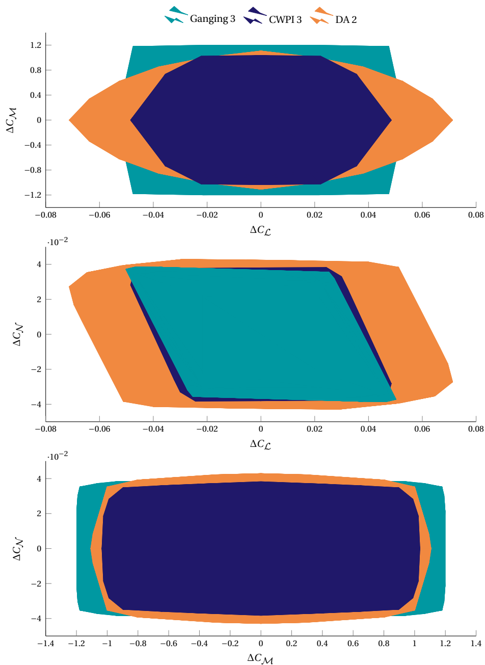
Figure 5.10 Comparison of the AASs corresponding to the optimal CS layouts obtained with each CA method. The legend entry refers to the CS layouts reported in Table 5.4.
