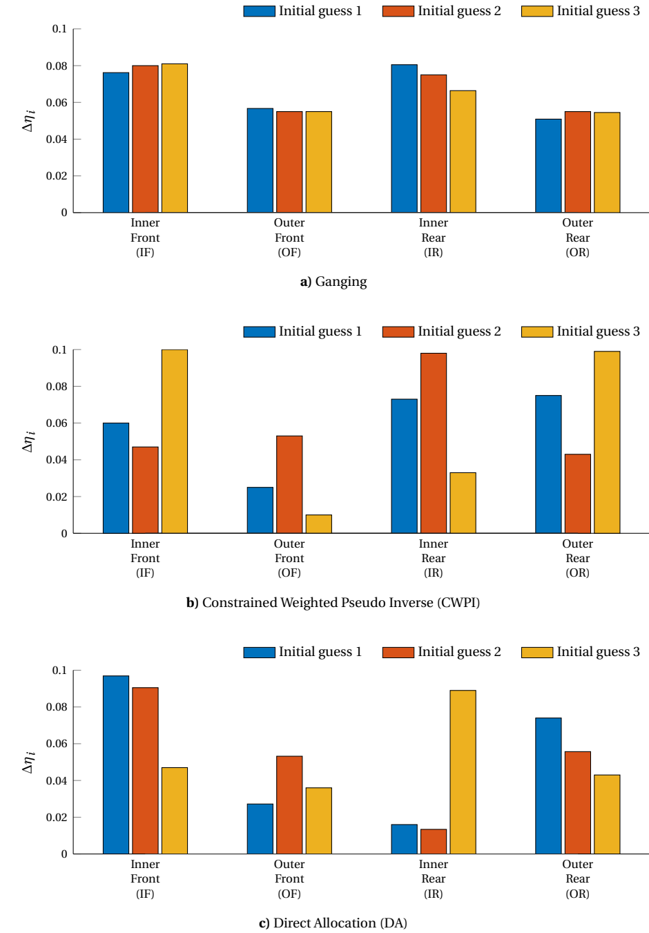
Figure 5.6 Comparison of optimal CS span widths for different CA methods and initial conditions. The legend refers to the initial conditions reported in Table 5.3.
