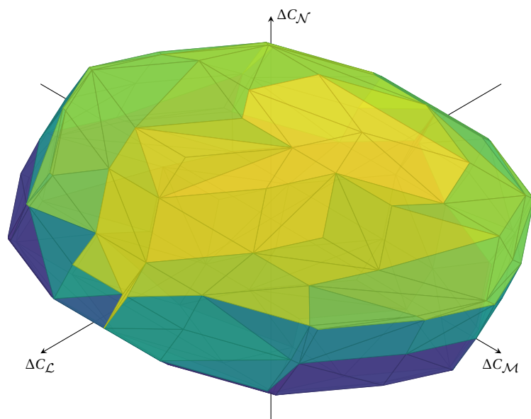
b) Effective Actions Set (EAS) in \mathbb{R}^3 : \mathbf{v} = [\Delta C_L, \Delta C_M, \Delta C_N]
