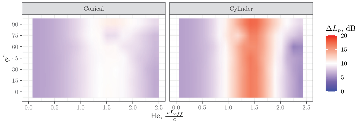
FIG. 13. (Color online) Acoustic response for conical cavity with \psi = 45^\circ and the straight walled cavity for incidence angles ( \phi ) from 0^\circ to 90^\circ . The cavities feature hard walls with no stainless steel cloth covering.
