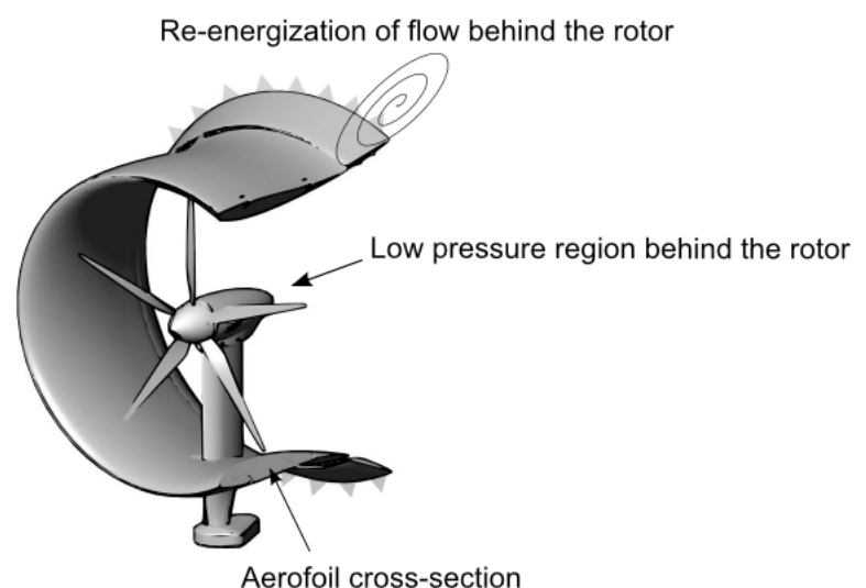
Figure 1 - Schematic of the ducted wind turbine with multi-element duct and trailing edge vortex generator.
