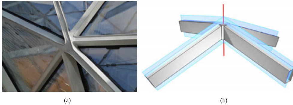
Figure 1.12: Nodes with torsion (a) and without torsion (b). [Source: Tellier et al., 2020]
