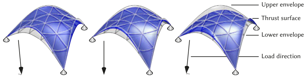
Figure 3.24: The envelopes defined by the thrust surfaces under various horizontal loads
