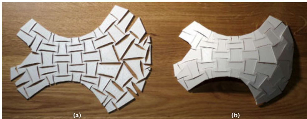
Figure 5.14: The 3D printed prototype of a free-form shell. (a) Flat configuration. (b) Curved configuration.
