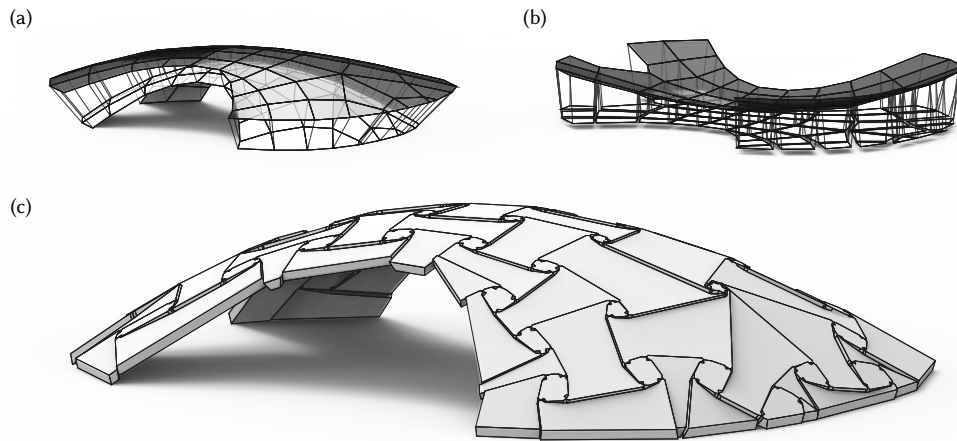
Figure 5.13: Geometric design of a free-form surface. (a–b) Unrolling the mesh panels with the neutral surface (gray transparent mesh). (c) Perspective view of the resulting mechanism. In the conical mesh, there is a six-edge node which is the umbilical point of the curved surface. The six-edge node becomes the hexagonal rotating connector in the mechanism.
