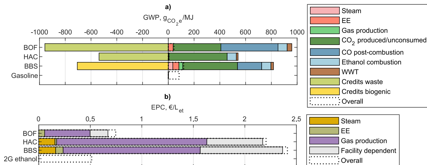
Fig. 4. Median values of the itemized contributions for (a) GWP and (b) EPC for the three process configurations. Gasoline is given a GWP equal to 83.3 \text{ gCO}_2\text{e}/\text{MJ} , while 2G ethanol production costs are taken as 0.51 \text{ €/L} (CGEE, 2017).
