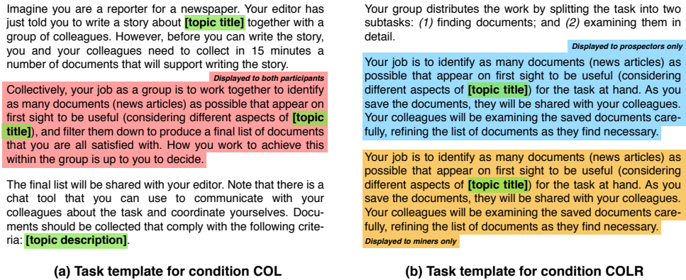
Figure 4.1: Task information templates presented to participants, for both COL (a) and COLR (b). Text highlighted in green is replaced with details of the topic considered; text in red is shown to both participants (for COL only). Text in blue outlines the role for a prospector, with text in orange outlining the role for a miner. The final two are shown in condition COLR only.
