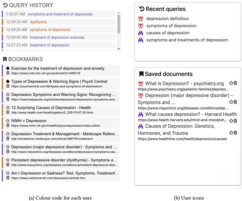
Figure 2.6: The SearchX collaborative components of recent queries and saved documents. On the left the components use the own style with colour coded and on the right with user icons generated with Identicon.js.
