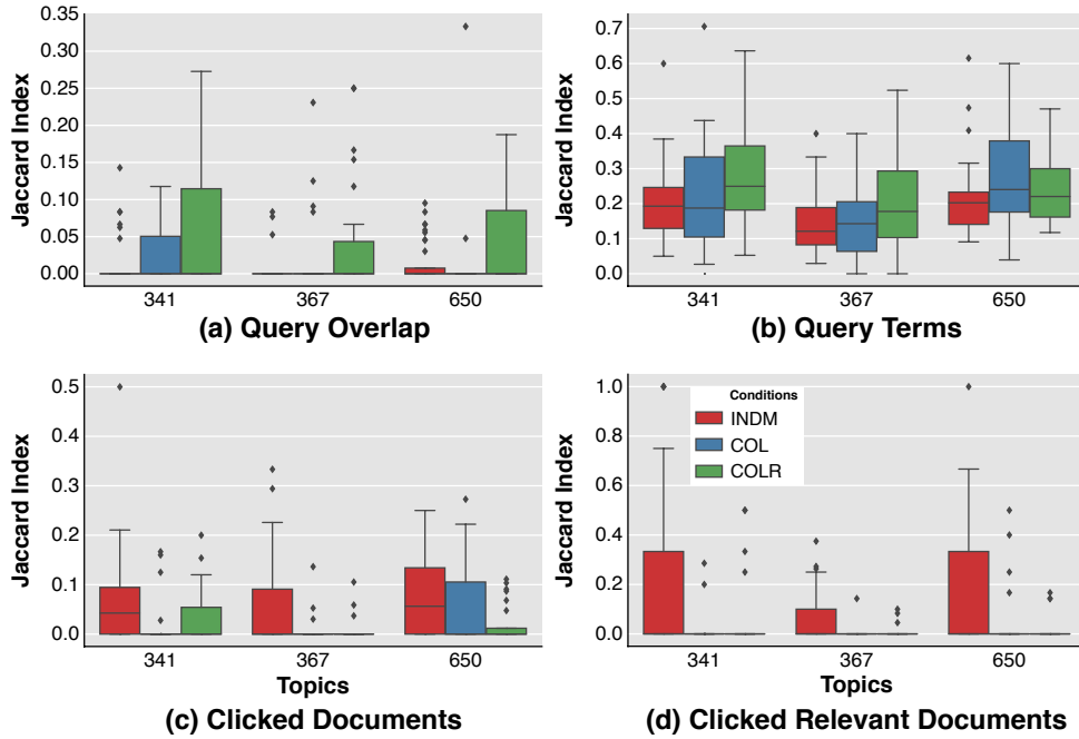
Figure 4.6: Overview of the Jaccard Index for the set of queries, query terms, clicks on documents, and clicks on documents that are relevant according to ROBUST05 relevance judgements between participants. Be aware of the different y-axis scaling.
