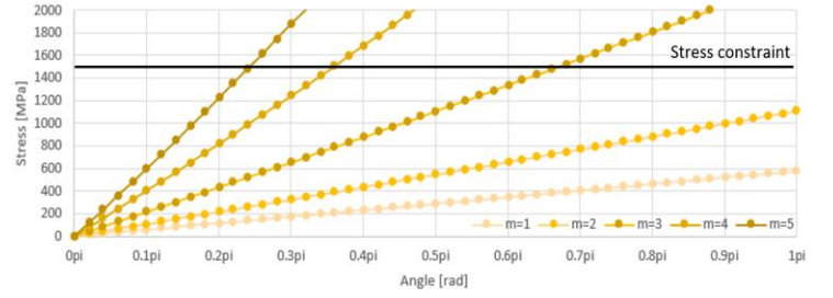
FIGURE 12: MAXIMUM VON MISES STRESS IN THE MIDDLE CELL OF THE FIRST ROW (M=1) FOR THE METAMATERIALS WITH 13 ARCS (N=13) AND DIFFERENT NUMBER OF ROWS WITH THE STEEL AISI 4340
