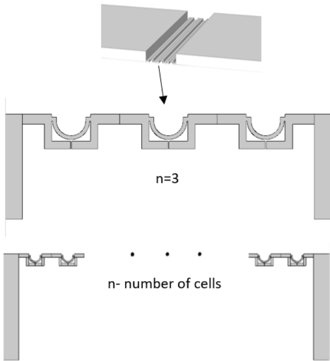
FIGURE 5: CONTACT-AIDED COMPLIANT ARRAYS WITH N -NUMBER OF CELLS
