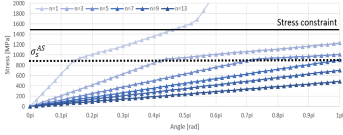
FIGURE 7: MAXIMUM VON MISES STRESS IN THE MIDDLE CELL OF THE ARRAY WITH NITI MATERIAL
