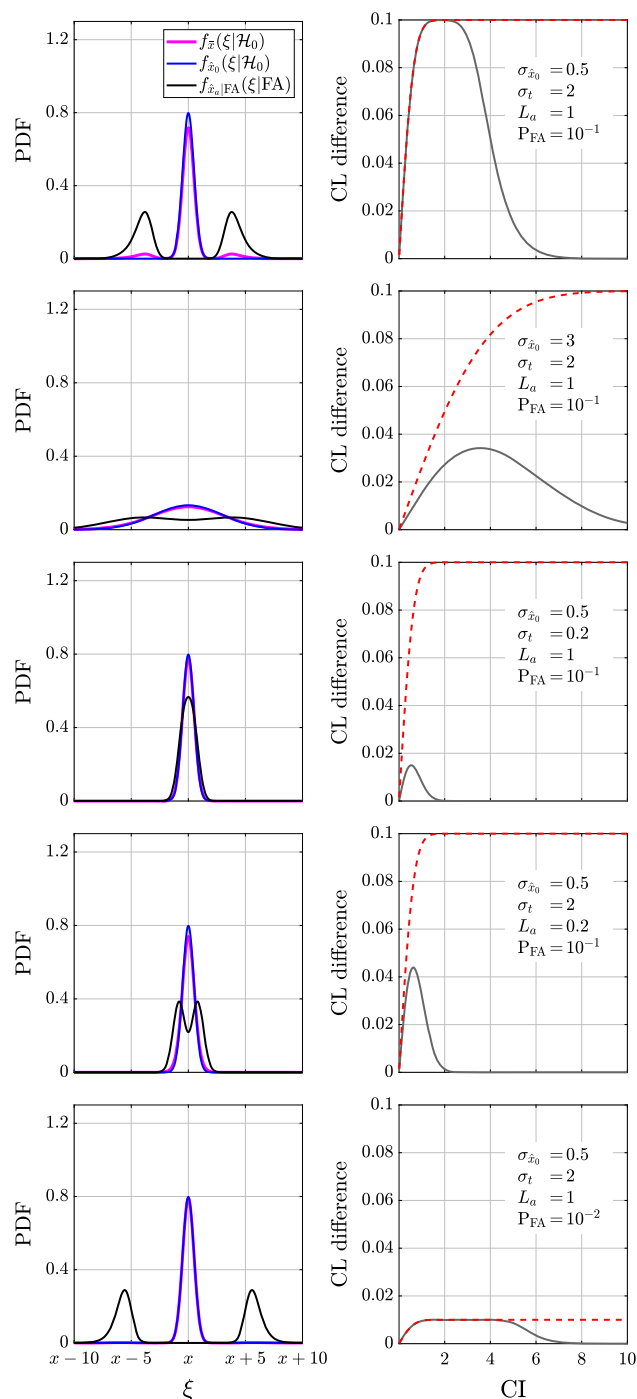
Fig. 5 [Left] Illustration of the DIA-estimator PDF under \mathcal{H}_0 and its components (cf. 10) for the models and conditions specified in (23) to (25). [Right] Illustration of the confidence level (CL) difference (1 - \alpha) - P(\bar{x} \in \mathcal{S}_\alpha^E(x)|\mathcal{H}_0) in gray and its upper bound (22) in red as a function of CI = \sqrt{\chi_{1-\alpha}^2(1,0)}\sigma_{\hat{x}_0} (26)
