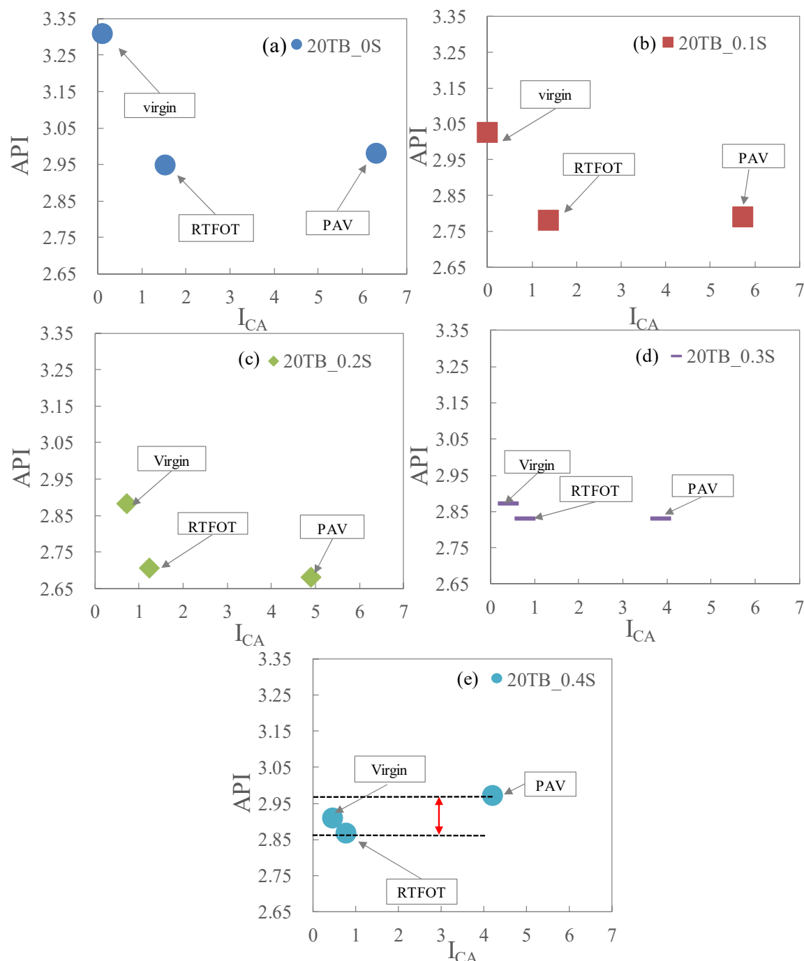
Figure 5. The relationship between I_{CA} and API: (a) 20TB_0S, (b) 20TB_0.1S, (c) 20TB_0.2S, (d) 20TB_0.3S, (e) 20TB_0.4S.
