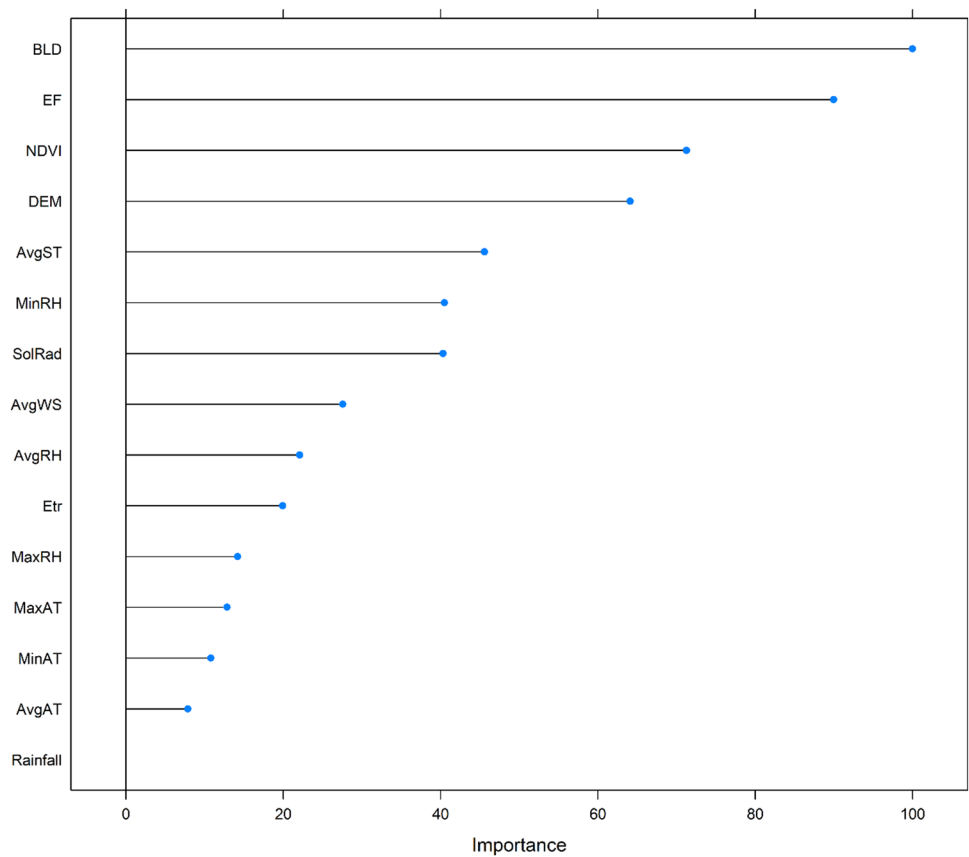
Fig. 5 Variable importance of RF model used in this study. Here, BLD is soil bulk density at each sensor location, AvgST is the daily average soil temperature, EF is the evaporation fraction, NDVI is normalized difference vegetation index, DEM is the digital elevation model, SolRad is the daily solar radiation, MinRH, MaxRH, and AvgRH are the minimum, maximum, and daily average relative humidity respectively, MaxAT, MinAT, and AvgAT are minimum, maximum, and daily average air temperatures, respectively, Etr is reference evapotranspiration, AvgWS is daily average wind speed, and rainfall is the sum of precipitation in that particular day
