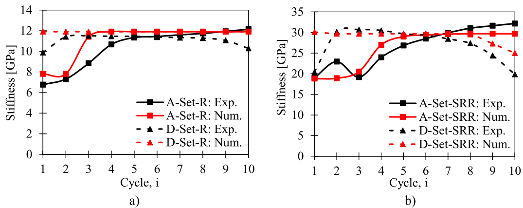
Fig. 25. Numerical and experimental stiffness: a) resin specimens; b) steel-reinforced resin specimens.
