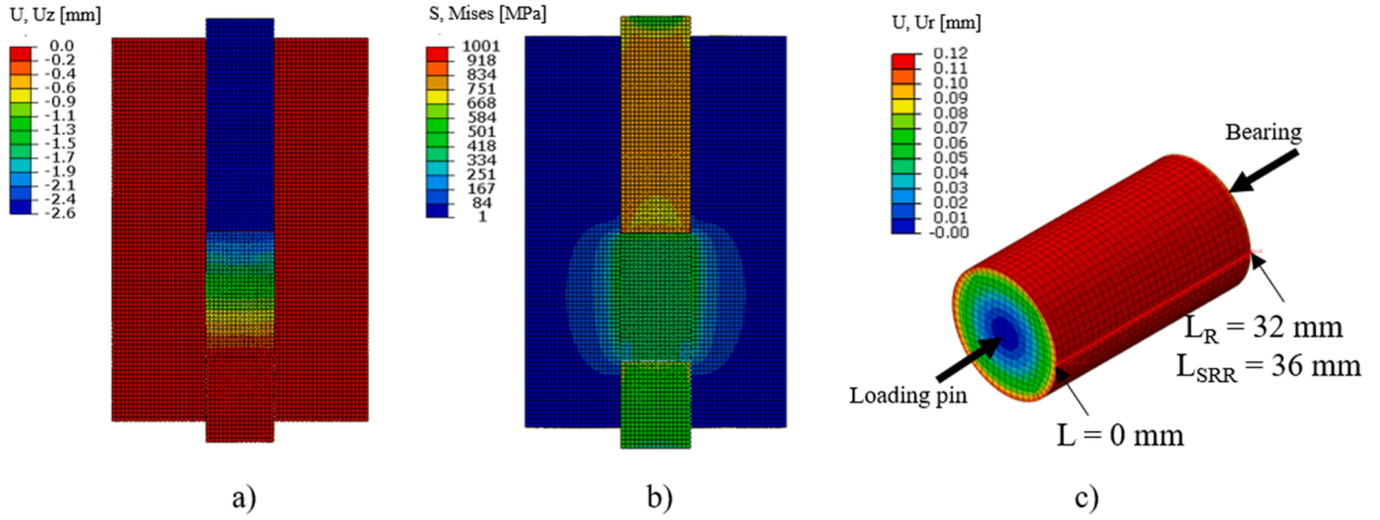
Fig. 18. Numerical results for resin specimen (A-Set) at maximum applied load of cycle 10: a) longitudinal deformation; b) von Mises stresses; c) radial deformation.
