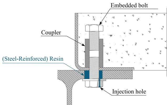
Fig. 1. Resin-injected bolted shear connector for demountable and reusable composite floor systems. Adapted from [17]
