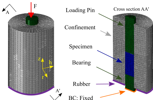
Fig. 17. Finite element model of confined material test.
