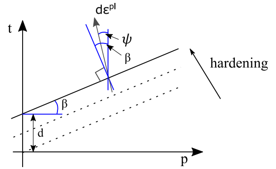
Fig. 4. Linear Drucker-Prager model: yield surface and flow direction in the p (hydrostatic pressure) - t (deviatoric stress) meridional plane [23].
