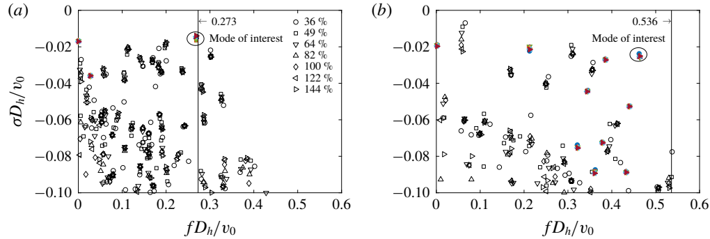
FIGURE 15. Eigenvalue spectrum for different mesh resolutions, where 100 % mesh resolution corresponds to reference mesh with resolution approximately equal to PIV mesh. Encircled eigenvalues correspond to selected mode of interest, coloured markers denote eigenvalues that are less or equally mesh-sensitive as the selected mode of interest (quantified via standard deviation) and vertical lines denote experimentally measured Strouhal number. (a) Mode m = 1 and (b) mode m = 2 .
