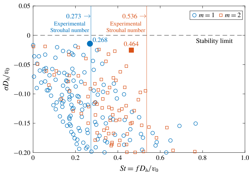
FIGURE 11. Eigenvalue spectrum with non-dimensional growth rate \sigma D_h/v_0 over Strouhal number St obtained by global direct LSA of the mean flow for azimuthal wavenumber m=1 and 2. Filled symbols (●, ■) denote the identified single-helical and double-helical modes, vertical solid lines denote the experimentally measured Strouhal numbers and the horizontal dashed line denotes the stability limit.
