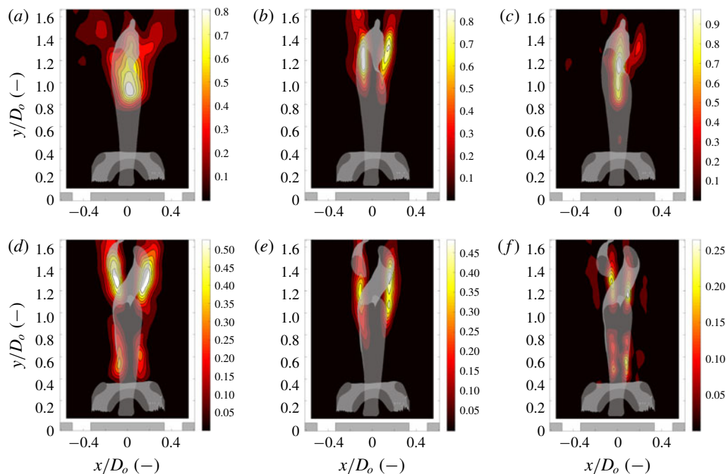
FIGURE 9. Coherent contribution to the second-order statistics of the single-helical ( a–c ) and double-helical ( d–f ) precession: ( a ) \overline{u'u'}/v_0^2 \times 100 ; ( b ) \overline{v'v'}/v_0^2 \times 100 ; ( c ) \overline{w'w'}/v_0^2 \times 100 ; ( d ) \overline{u'u'}/v_0^2 \times 100 ; ( e ) \overline{v'v'}/v_0^2 \times 100 ; ( f ) \overline{w'w'}/v_0^2 \times 100 .
