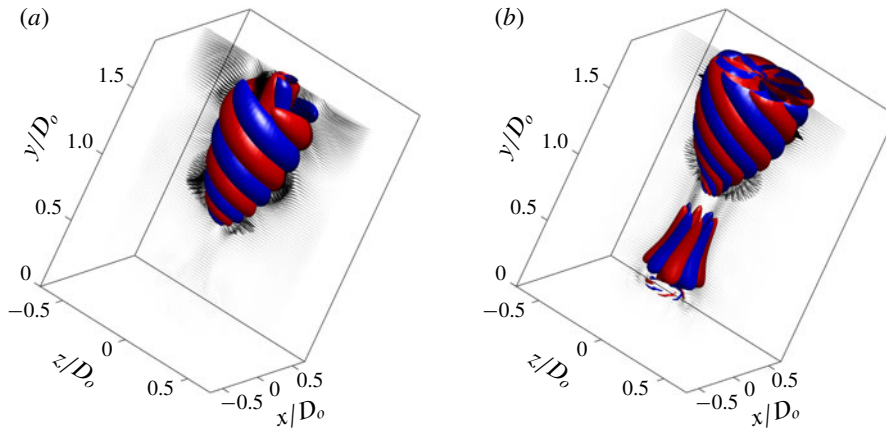
FIGURE 12. Spatial structure of the identified PVC modes obtained by global direct LSA; isosurface of Q criterion (arbitrary scale and arbitrary phase angle); blue, real part; red, imaginary part. Vector field shows the real part of the coherent fluctuations projected onto the plane x=0 . (a) Single-helical mode ( m=1 ). (b) Double-helical mode ( m=2 ).
