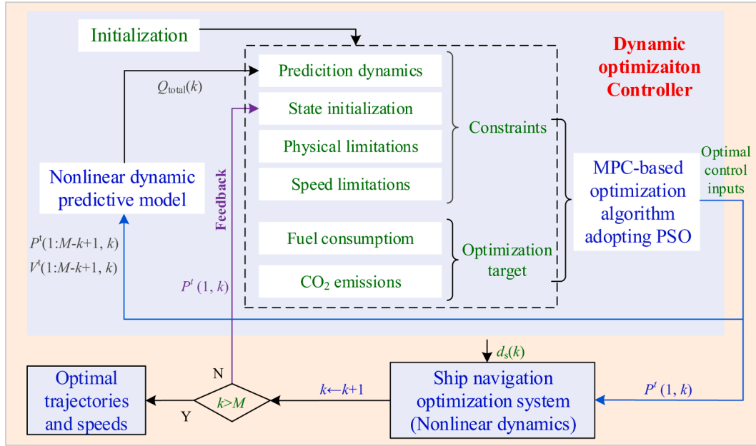
Fig. 11. A schematic diagram of the dynamic collaborative optimization controller.
