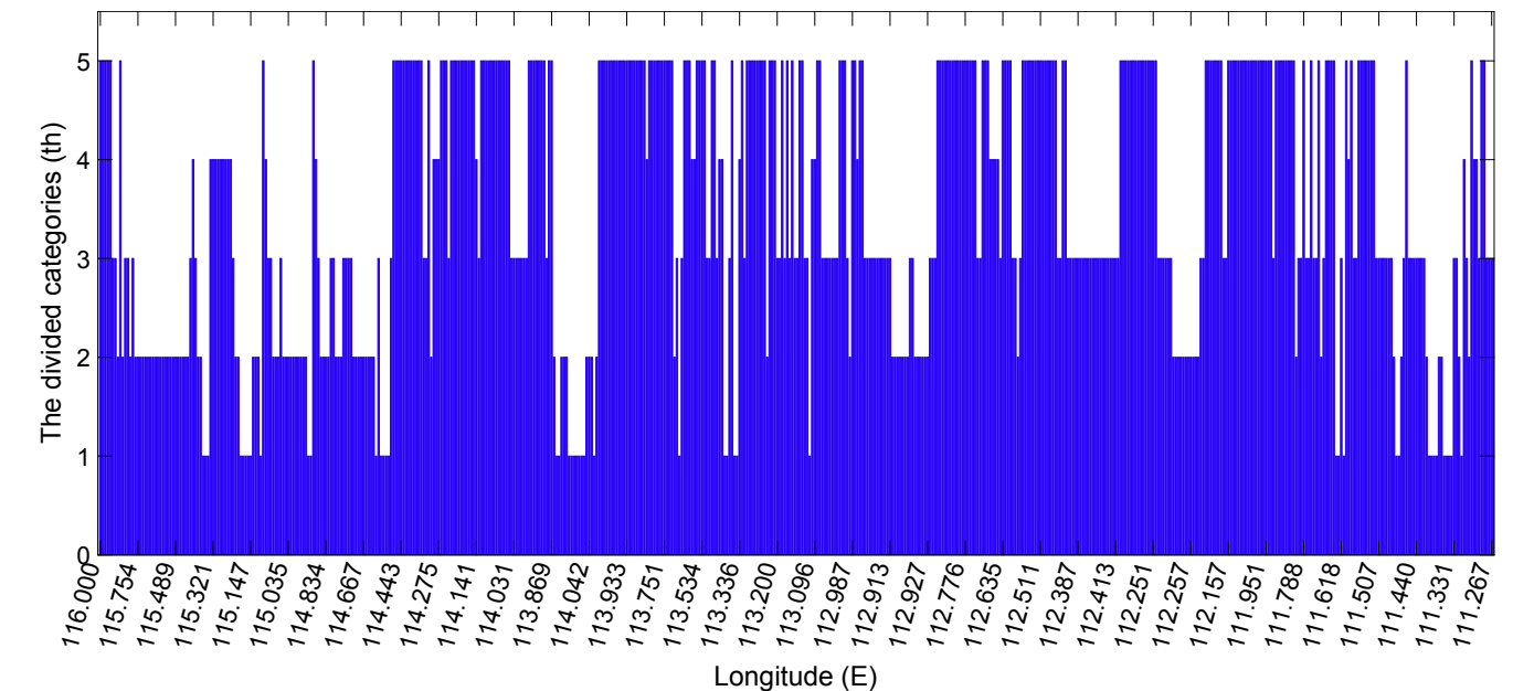
Fig. 11. Categories of environment at different locations of the middle reach (Rain season).
