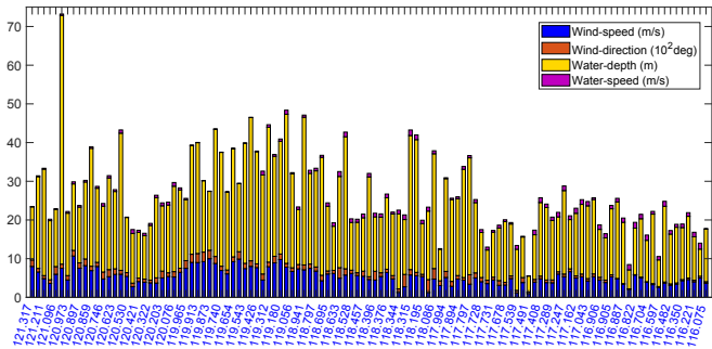
Fig. 4. Average environmental data at different locations of the lower reach.
