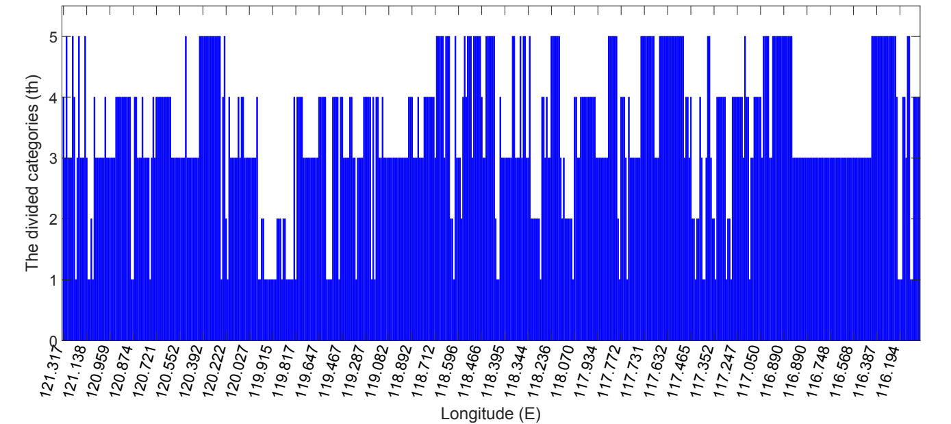
Fig. 10. Categories of environment at different locations of the lower reach (Rain season).
