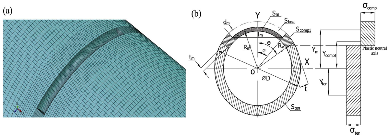
Fig. 5. (a) schema of mesh distribution of notched region; (b) sketch of pipe cross-section with notch and notch parameters.
