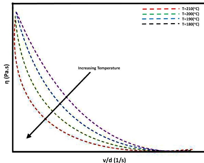
Figure 4. Correlation between printing speed/tube filament diameter and shear viscosity.
