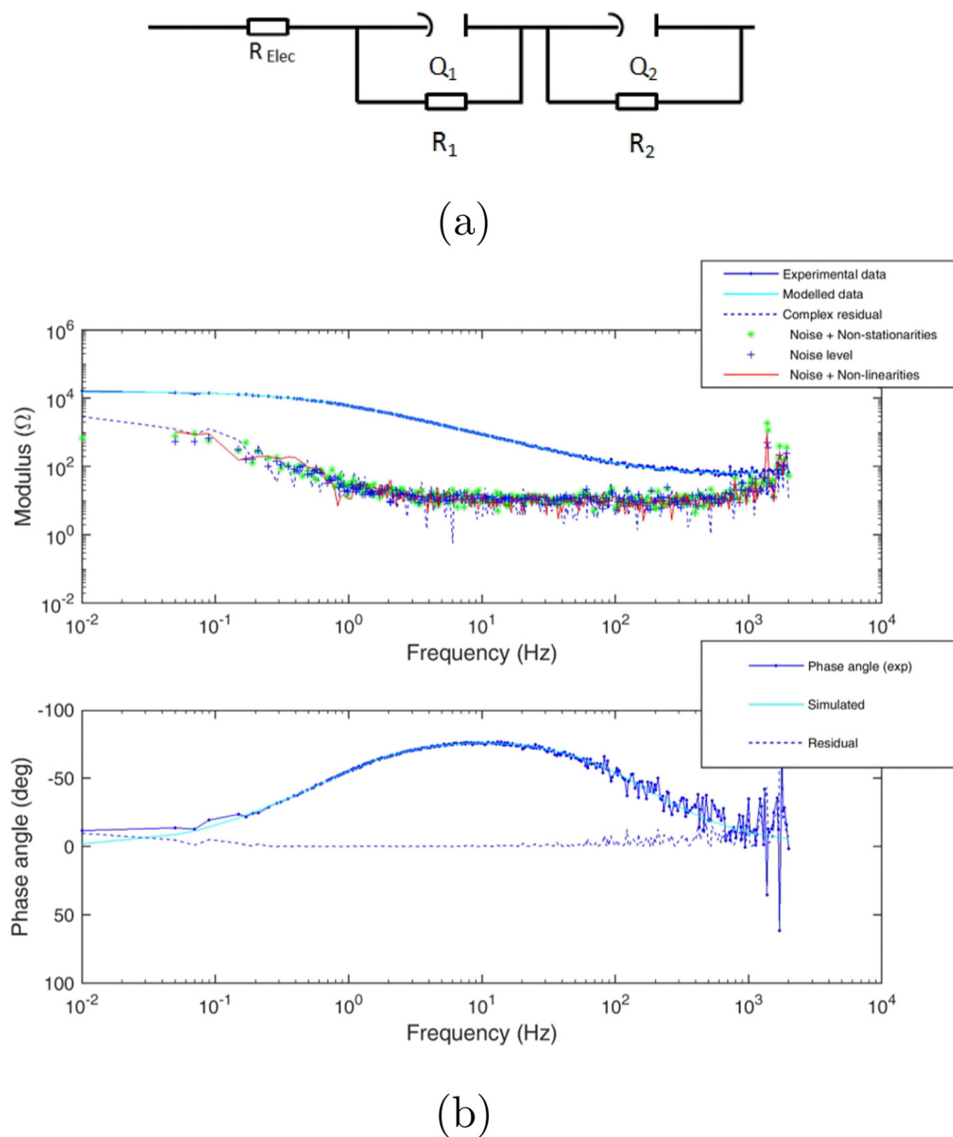
Fig. 7. (a) Equivalent electrical circuit to describe the PAA coating on aluminum oxide. The first time constant describes the organic layer (resistance R_1 and constant phase element Q_1 ), the second time constant describes the aluminum oxide layer response (resistance R_2 and constant phase element Q_2 ). (b) Bode magnitude and phase plot containing the experimental data, modelled curve, complex residual, noise levels, noise on the excited frequencies and noise on the non-excited frequencies of the measurement at 1 h of exposure to the electrolyte.
