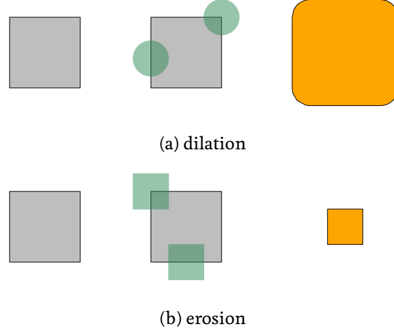
Figure 9: Two morphological operators in 2D applied on A (dark grey) with a structuring element B (green), the result is the orange subset of \mathbb{R}^2 .
