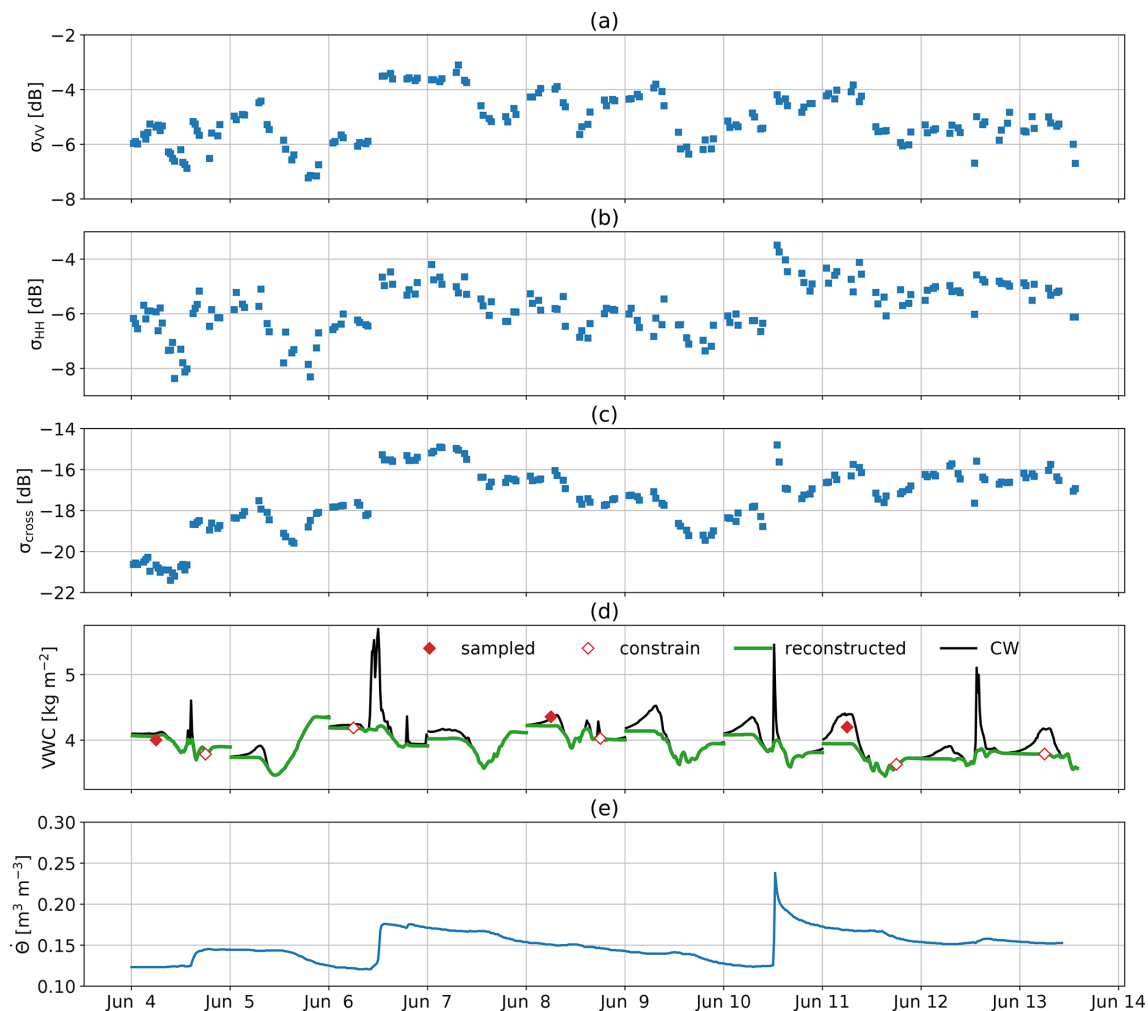
Figure 9. Full polarimetric L-band backscatter and separated effects for a 10 d period near the end of the growing season in 2018, with (a) VV-polarized scattering coefficient, (b) HH-polarized scattering coefficient, and (c) averaged VH- and HV-polarized scattering coefficients, (d) sampled and reconstructed VWC, total canopy water, which is the sum of reconstructed VWC and SCW, and (e) soil moisture at 5 cm depth. The measurements which are used to constrain the reconstructed line are accentuated with open markers.
