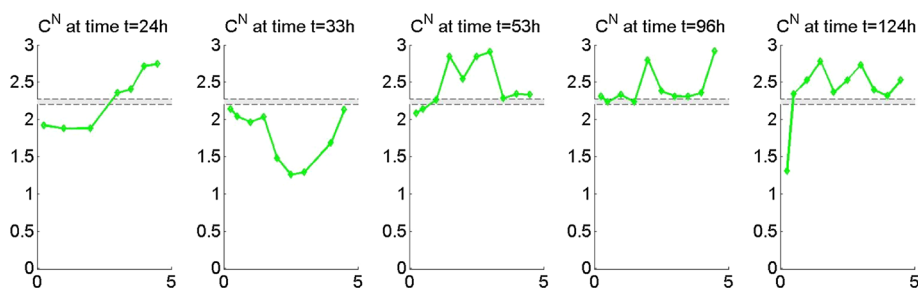
Fig. 4 Concentration of nitrogen [ C^N (kmol/m 3 )] in the column [distance in (m)] at several times (green line) and the theoretical bandwidth for this concentration (two dotted horizontal lines)
