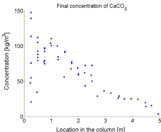
Fig. 3 Concentration of calcium carbonate (kg/m 3 ) in the column at the end of the experiment
