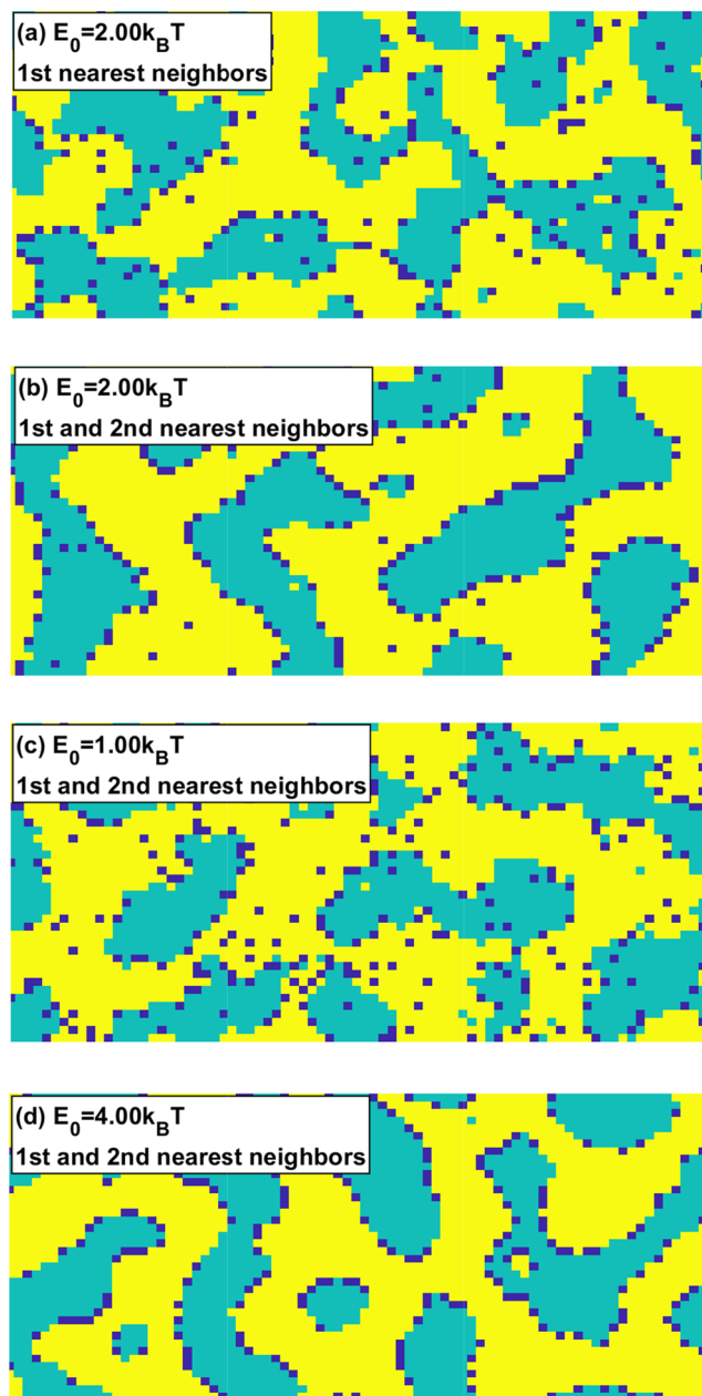
FIG. 6. Island formation between two species A and B with different energetic interaction ( E_0 ) between two adjacent inter-species and taking into account different neighbors. The yellow, green, and blue color represent A, B, and vacant sites, respectively.
