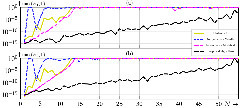
Figure 5.5: Results of example ‘Non-zero background potential’ (Section 5.5.4). The target potentials, with 2 + N eigenvalues, were computed with three benchmark algorithms (—/····/—·—) and the proposed one (—). The errors E_1 and E_2 were calculated with (5.60) for N \in \mathbb{N}_1^{55} .
