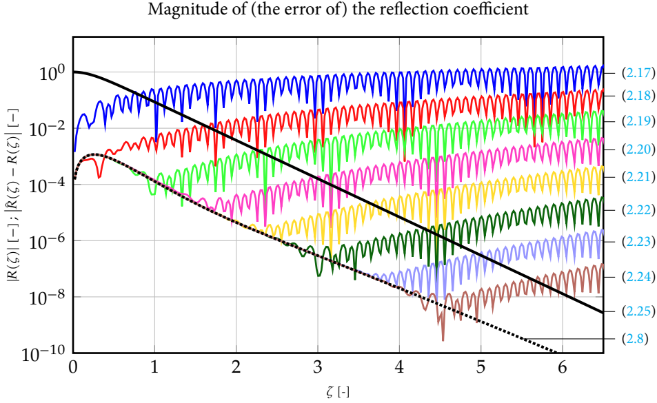
Figure 2.1: The black solid curve with label (2.25) shows the magnitude of the reflection coefficient of a squared hyperbolic secant potential for the KdV. All other curves show the magnitude of the error of a numerical approximation of the reflection coefficient. The numbers between brackets refer to the corresponding equation: (2.8): error without splitting (due to staircase approximation), (2.17)–(2.24): error with splitting.
