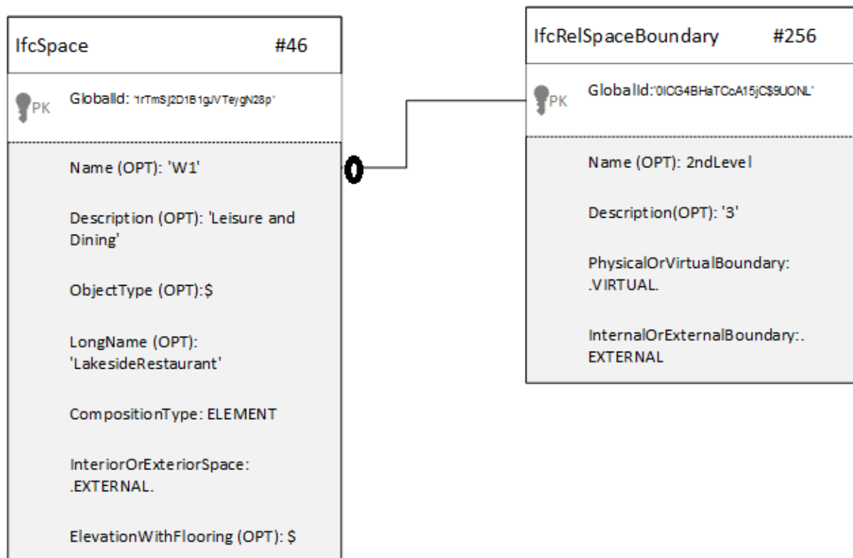
Figure 9. Extract from IFC model showing IfcSpace with attributes for a conceptual mass of the Lake Restaurant. The '3' in the IfcRelSpaceBoundary entity represents a proposed new description for an ambulatory boundary and replaces the original '2a'
