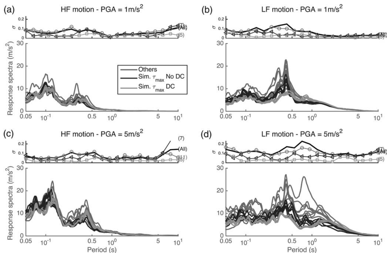
Figure 18. Comparison of the pseudoacceleration RS at the ground surface of P1 with rigid substratum condition, for the NL computation using for (a) and (c) graphs the HF input motion and for (b) and (d) graphs the LF input motion and with for the (a) and (b) graphs the middle input motion PGA and the (c) and (d) graphs the highest input motion PGA. The RS were sorted according to three groups: group 1 is composed of the code/team couples using similar \tau_{\max} and damping control constitutive model, group 2 use similar \tau_{\max} and no damping control, and group 3 are the other code/team couples. The standard deviation for each subgroup is compared with the standard deviation using all results in the upper graphs, the figures indicate the number of simulations that are in each group.
