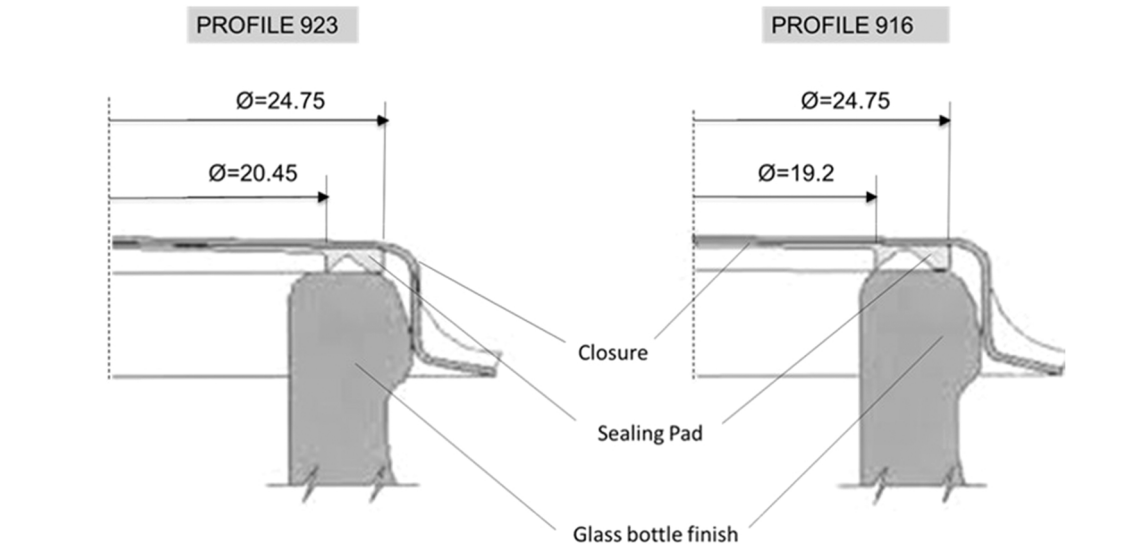
Fig. 1. Two different pry-off double lip profile.
