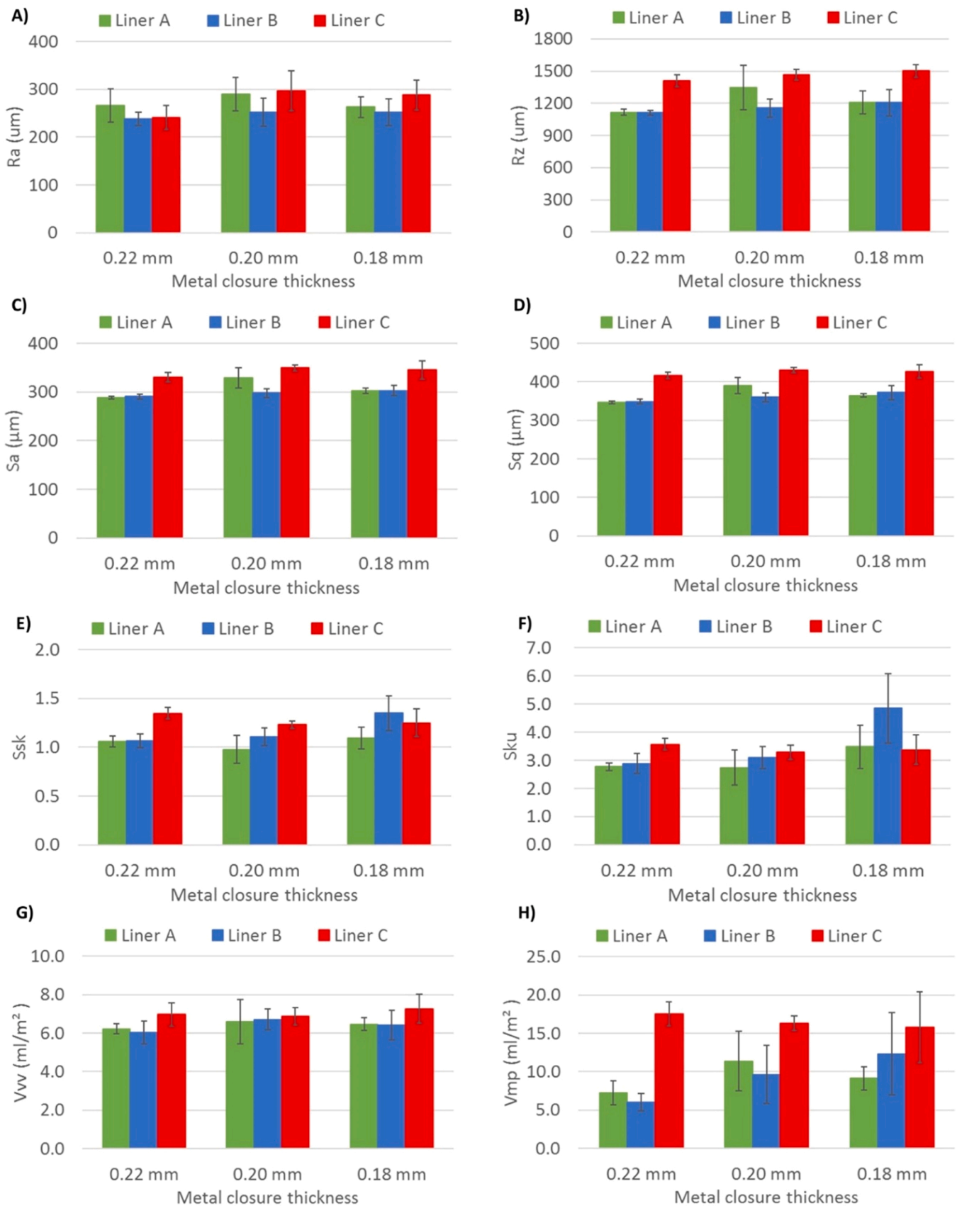
Fig. 6. Line and surface roughness parameters of different liners sealed in metal caps of a different thicknesses a) R_a (arithmic mean surface roughness), b) R_z (surface roughness depth), c) S_a (arithmetical mean height), d) S_q (root mean square height), e) S_{sk} (skewness), f) S_{ku} (kurtosis), g) V_{vv} (average void volume), h) V_{mp} (peak material volume).
