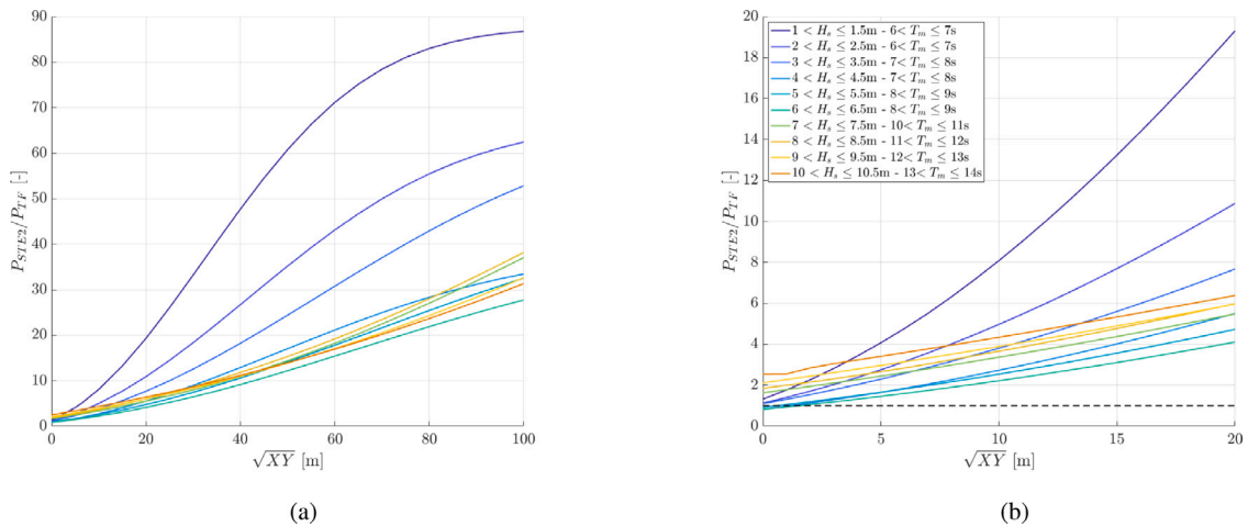
Fig. 5. Comparison of the STE2 (Benetazzo et al. (2015)) and TE Tayfun-Fede (Tayfun and Fede, 2007) estimate of P(\eta_{max}/\sigma \geq 5 | D) with D = 1200 s. (a) Area sizes ranging from no spatial component ( X = 0, Y = 0 ) to 100 \times 100 m 2 . (b) Area sizes ranging from no spatial component ( X = 0, Y = 0 ) to 20 \times 20 m 2 . The horizontal black dashed line visualizes a y-ratio of 1.
