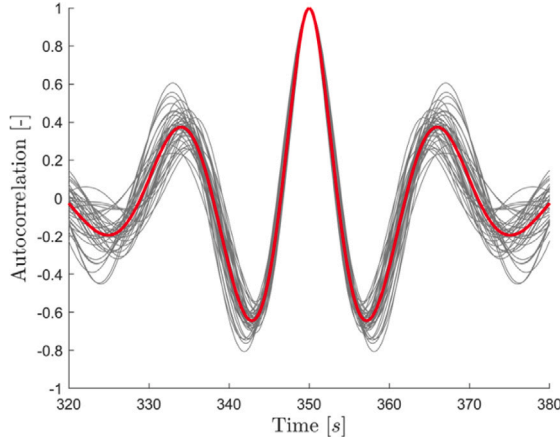
Fig. 9. A visual representation of the most-likely rogue wave shape for the third rogue wave threshold H_{\text{rogue}} \geq 18.26 m.
