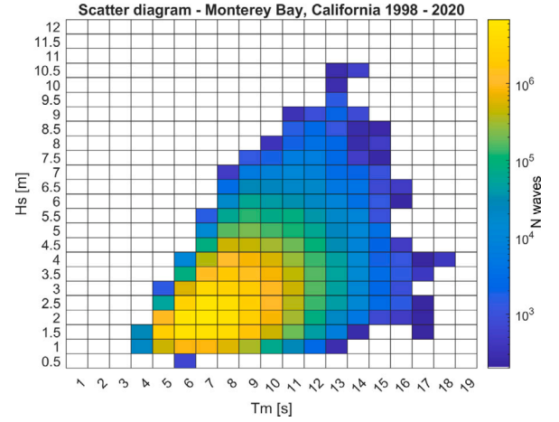
Fig. 2. Scatter diagram of the significant wave height and the mean zero-crossing wave period.
