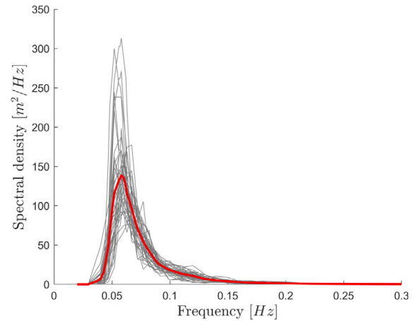
Fig. 8. A visual representation of the most-likely wave spectrum for the third rogue wave threshold H_{\text{rogue}} \geq 18.26 m.
