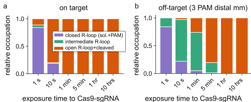
Fig. 6 Dynamics among metastable states resemble structural dynamics. a ) Time-resolved relative occupancy for the on-target among the closed R-loop state (solution and PAM bound), the intermediate R-loop state, and the open R-loop and cleaved state (c.f. Fig. 2d of Dagdas et al. 51 ); b ) Relative occupancy at different time points for an off-target with the last 3 PAM distal base pairs mismatched (c.f. Fig. 2f of Dagdas et al. 51 ).
