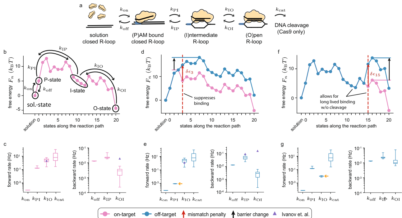
Fig. 5 Metastable states control the targeting dynamics. a ) A coarse-grained version of the reaction scheme shown in Fig. 1a. Apart from the unbound and post-cleavage state, the targeting-reaction pathway is reduced to just three states: PAM bound and R-loop closed (0 bp hybrid), intermediate R-loop (7–13 bp hybrid), and open R-loop (20 bp hybrid). b ) Microscopic free-energy landscape for the on-target exposed to 1 nM (d)Cas9-sgRNA (Fig. 4a) with coarse-grained states and rates indicated in black. c ) The calculated (see Methods) coarse-grained forward and backward rates on the on-target. Purple triangles are rates from Ivanov et al. 42 , when available at zero torque. d ) Microscopic free-energy landscape for an off-target with a mismatch at position 3 (blue), together with the on-target free-energy landscape (pink). Red arrow indicates the free-energy penalty \delta\epsilon_3 at the mismatch, and black arrow indicates the resulting shift in barrier height. e ) The calculated coarse-grained forward and backward rates on an off-target with a mismatch at position 3. Orange arrow highlights the rate that changed considerably compared to on-target. Purple triangles are rates from Ivanov et al. 42 , when available at zero torque. f ) Microscopic free-energy landscape for an off-target with a mismatch at position 15 (blue), together with the on-target free-energy landscape (pink). Red arrow indicates free-energy penalty \delta\epsilon_{15} at the mismatch, and black arrow indicates the resulting shift in barrier height. g ) The calculated coarse-grained forward and backward rates on an off-target with a mismatch at position 15. Orange arrow highlights the rate that changed considerably compared to on-target. In Fig. 5c, e, and g, central line represents the median, the box plots represent the interquartile range, and whiskers represent the full range among our 33 near equivalent solutions.
