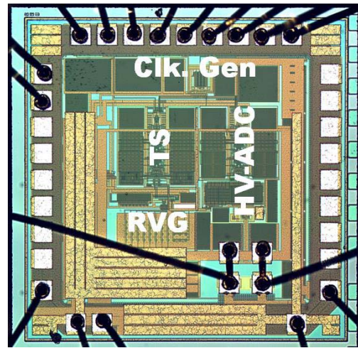
Fig. 7. Chip photograph.
