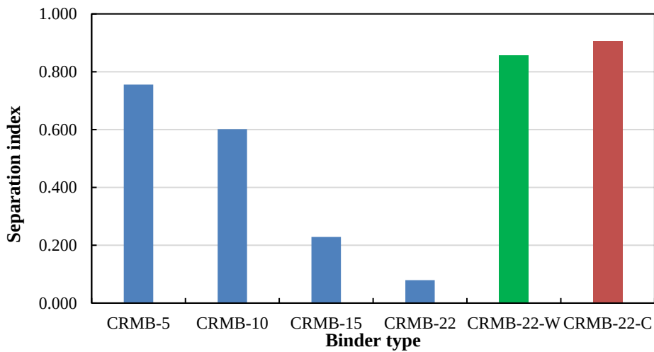
Figure 6.29 Separation index of different binders.
