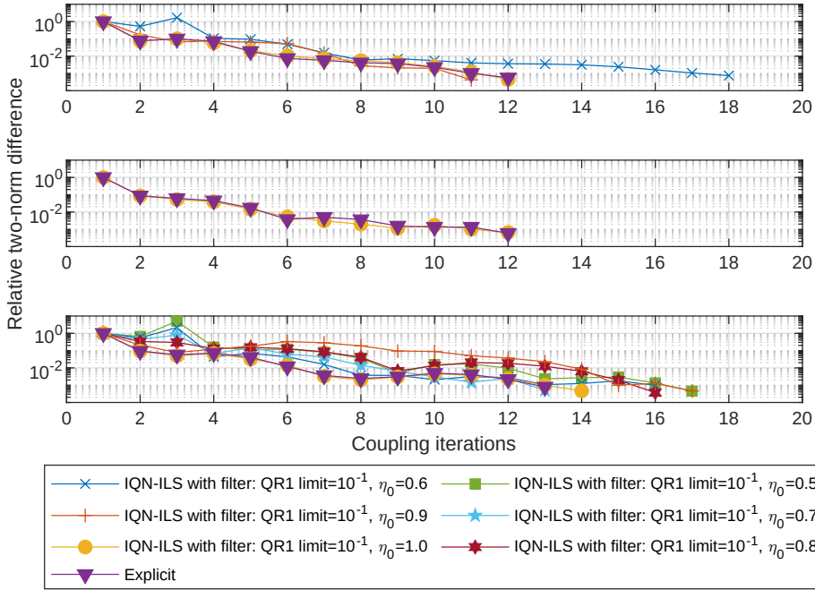
Figure 4.8: Relative two-norm convergence of the interface deformation vector during FSI simulation. Top figure corresponds to coarse mesh density, middle to medium, and bottom figure to finest mesh density.
