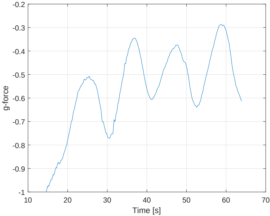
Figure 4.5: Normalised g-force in yaw-axis direction during power phase to illustrate plunging motion of the wing. Next to the periodic acceleration due to the reel-out manoeuvre small oscillations can be observed.
