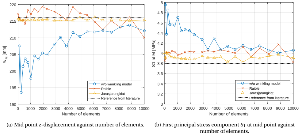
Figure 3.7: Mesh sensitivity
