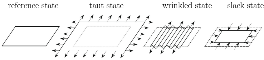
Figure 2.7: Different membrane states - reference, taut, wrinkled, and slack [41]
