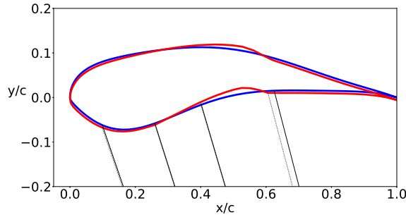
Figure 5.6: Undeformed (blue) and deformed (red) rib geometry with wrinkling model employed.
