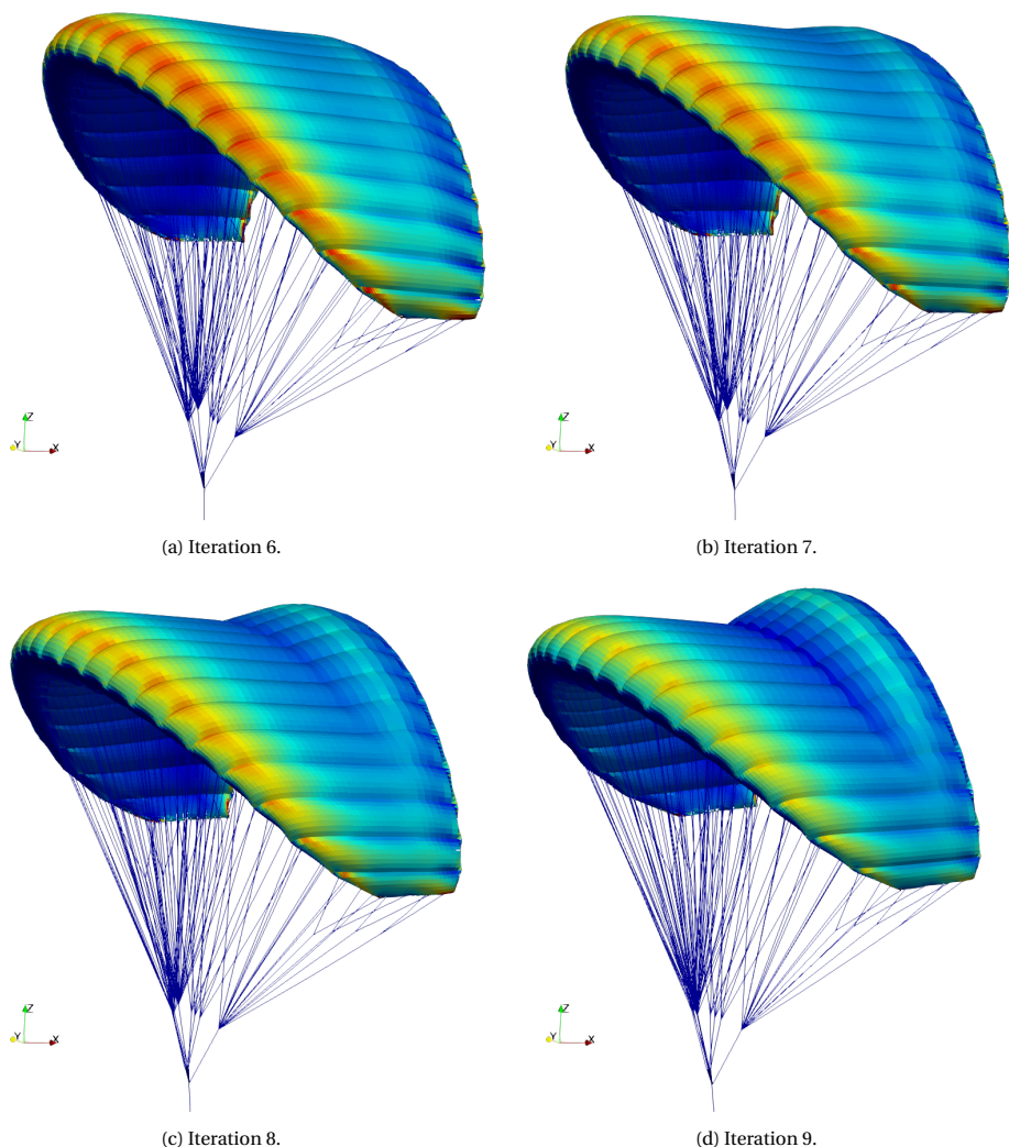
Figure 4.27: FSI divergence with explicit coupling on fine mesh density (iterations 6-9).
