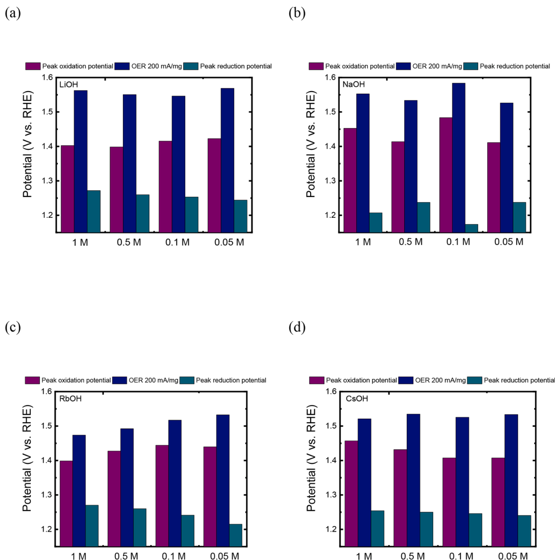
Fig. 2. Peak oxidation (purple) and reduction (green) potential of the Ni(OH) 2 /NiOOH redox couple and the potential at which 200 mA/mg for OER (blue) is reached for different electrolyte compositions. (a) LiOH, (b) NaOH, (c) RbOH, and (d) CsOH additions to a KOH electrolyte. Data from cyclic voltammograms of a Ni(OH) 2 film deposited on a GC-RDE at 1600 rpm.
